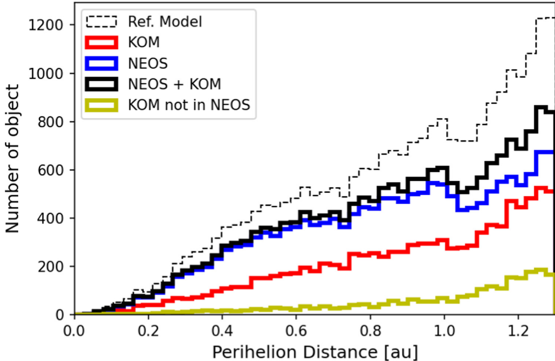
Figure 16. from Tommy Grav et al 2023 Planet. Sci. J. 4 doi:10.3847/PSJ/ad072e https://dx.doi.org/10.3847/PSJ/ad072e © 2023. The Author(s). Published by the American Astronomical Society.
