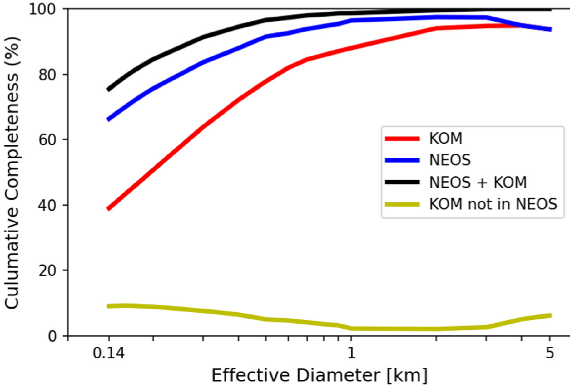
Figure 14. from Tommy Grav et al 2023 Planet. Sci. J. 4 doi:10.3847/PSJ/ad072e https://dx.doi.org/10.3847/PSJ/ad072e © 2023. The Author(s). Published by the American Astronomical Society.
