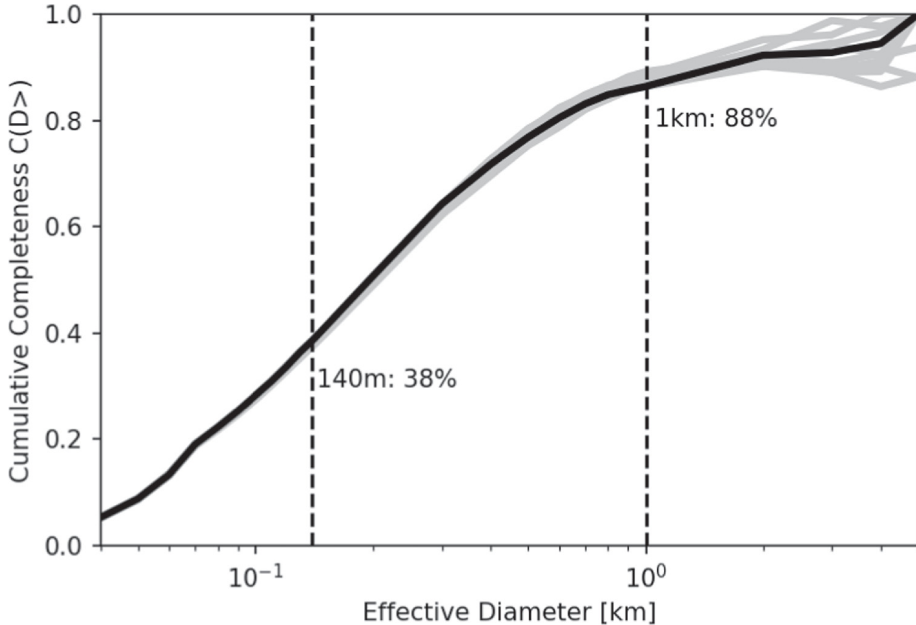
Figure 12. from Tommy Grav et al 2023 Planet. Sci. J. 4 doi:10.3847/PSJ/ad072e https://dx.doi.org/10.3847/PSJ/ad072e © 2023. The Author(s). Published by the American Astronomical Society.
