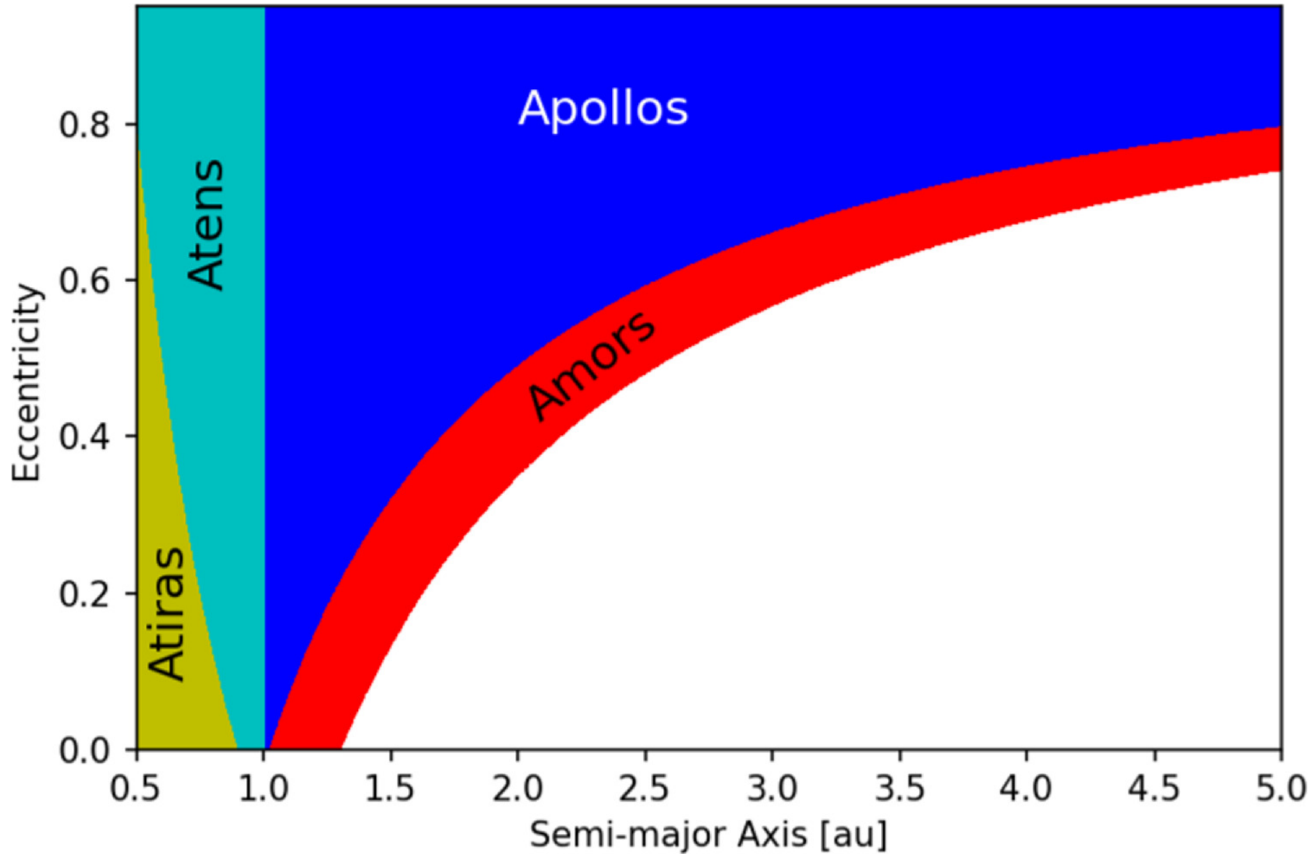
Figure 1. from Tommy Grav et al 2023 Planet. Sci. J. 4 doi:10.3847/PSJ/ad072e https://dx.doi.org/10.3847/PSJ/ad072e © 2023. The Author(s). Published by the American Astronomical Society.
