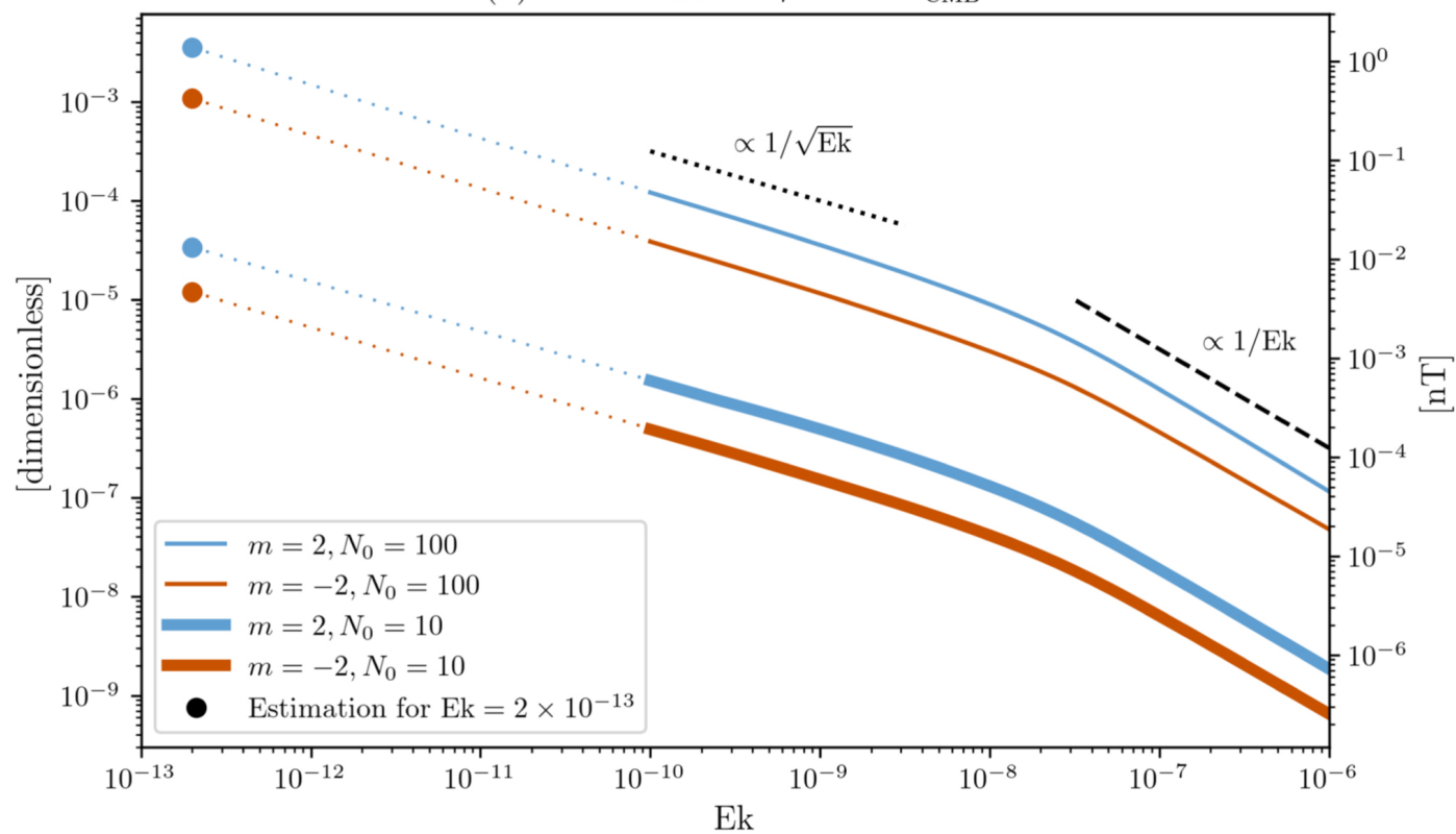
(b) r.m.s. value of b_r at r = r_{\text{CMB}}
