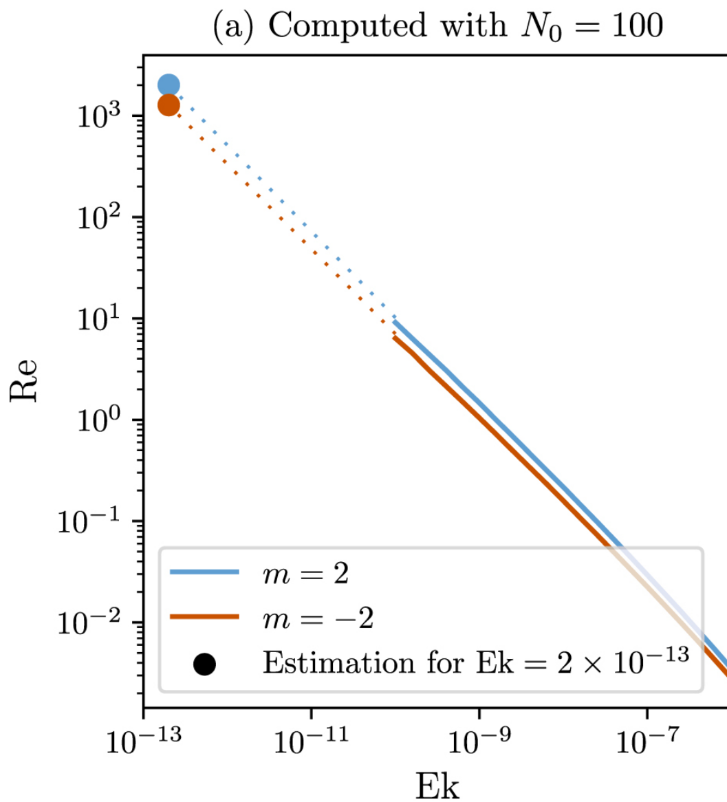
Figure 8. from Fleur Seuren et al 2023 Planet. Sci. J. 4 doi:10.3847/PSJ/acee77 https://dx.doi.org/10.3847/PSJ/acee77 © 2023. The Author(s). Published by the American Astronomical Society.
