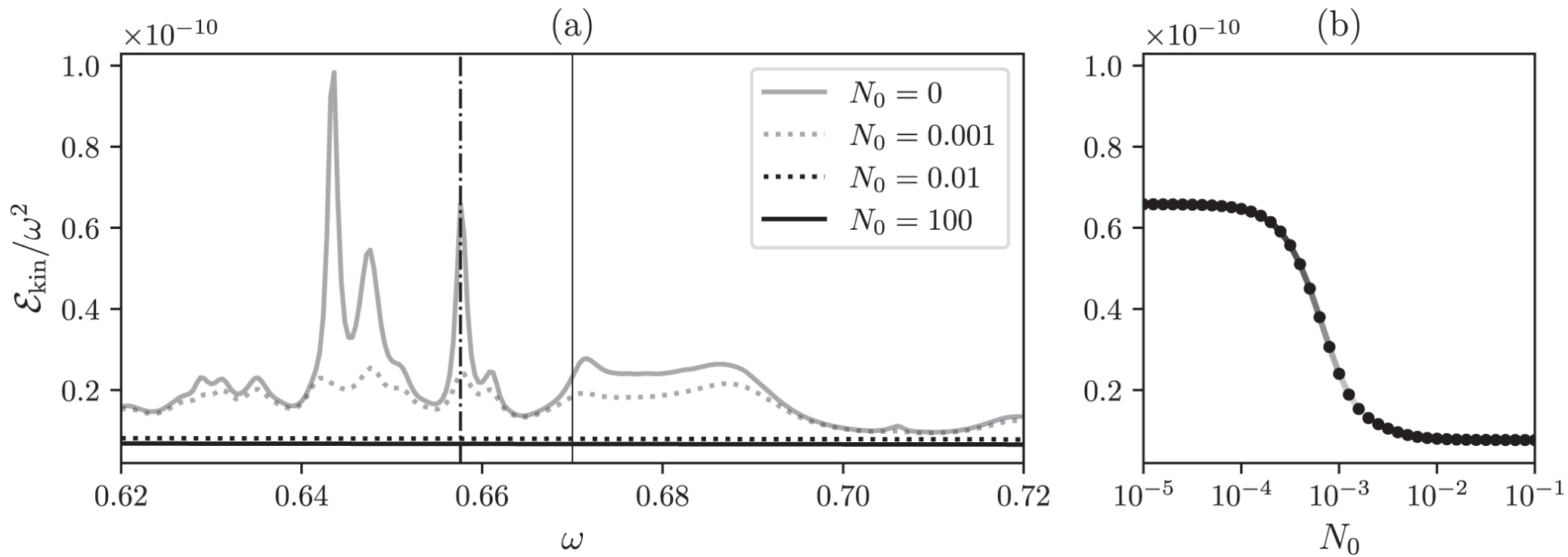
Figure 5. from Fleur Seuren et al 2023 Planet. Sci. J. 4 doi:10.3847/PSJ/acee77 https://dx.doi.org/10.3847/PSJ/acee77 © 2023. The Author(s). Published by the American Astronomical Society.
