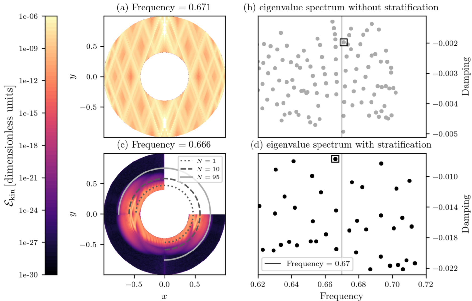
Figure 4. from Fleur Seuren et al 2023 Planet. Sci. J. 4 doi:10.3847/PSJ/acee77 https://dx.doi.org/10.3847/PSJ/acee77 © 2023. The Author(s). Published by the American Astronomical Society.
