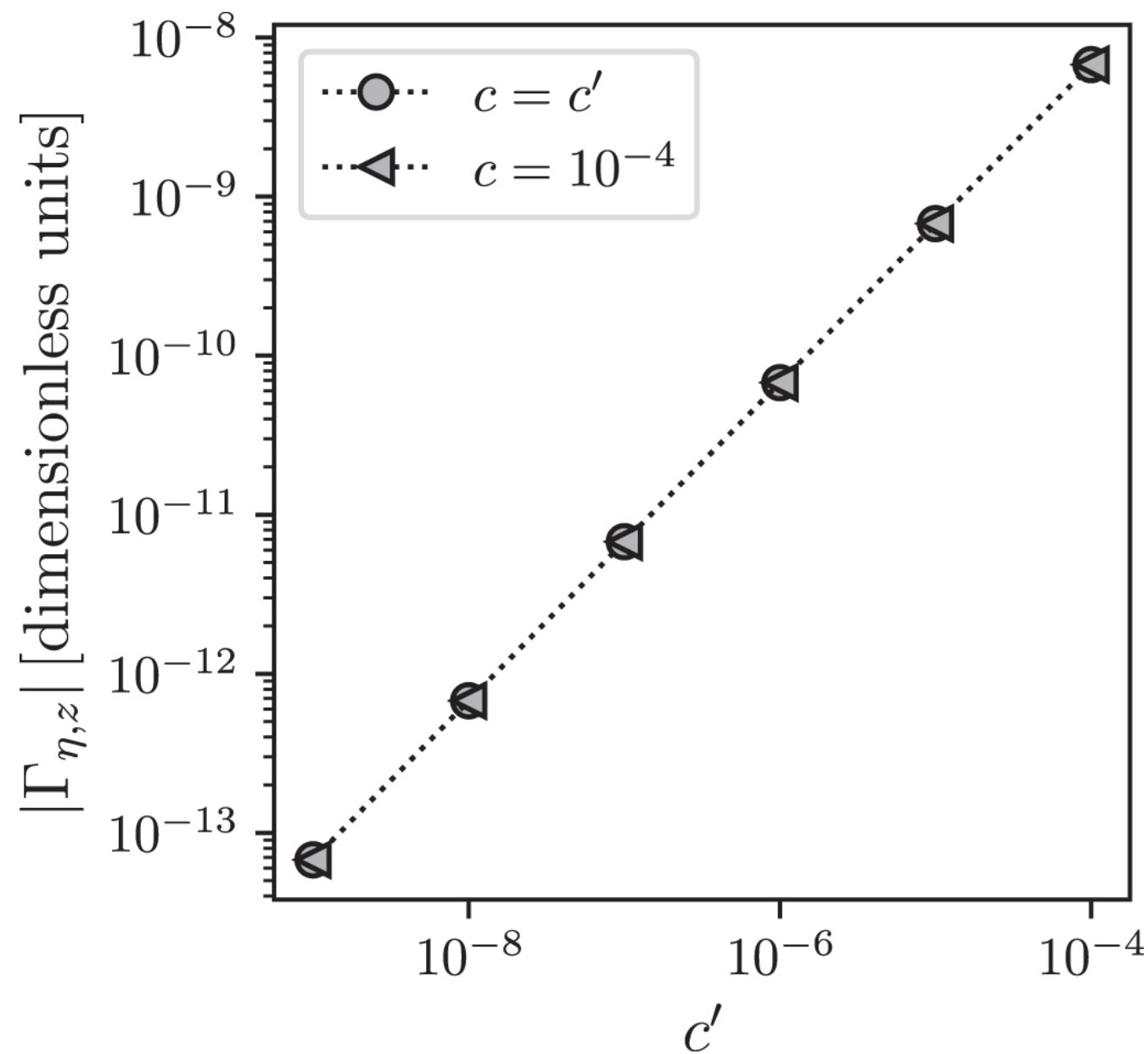
Figure 2. from Fleur Seuren et al 2023 Planet. Sci. J. 4 doi:10.3847/PSJ/acee77 https://dx.doi.org/10.3847/PSJ/acee77 © 2023. The Author(s). Published by the American Astronomical Society.
