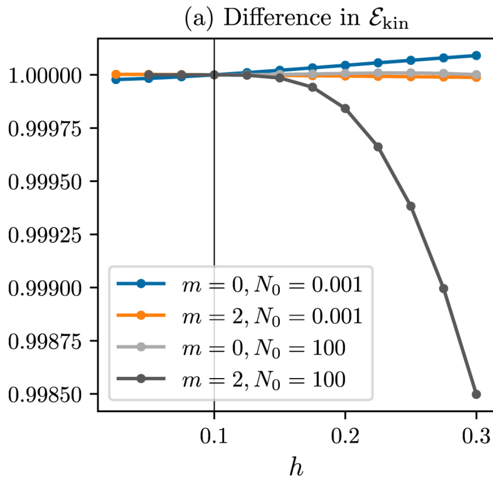
Figure 10. from Fleur Seuren et al 2023 Planet. Sci. J. 4 doi:10.3847/PSJ/acee77 https://dx.doi.org/10.3847/PSJ/acee77 © 2023. The Author(s). Published by the American Astronomical Society.
