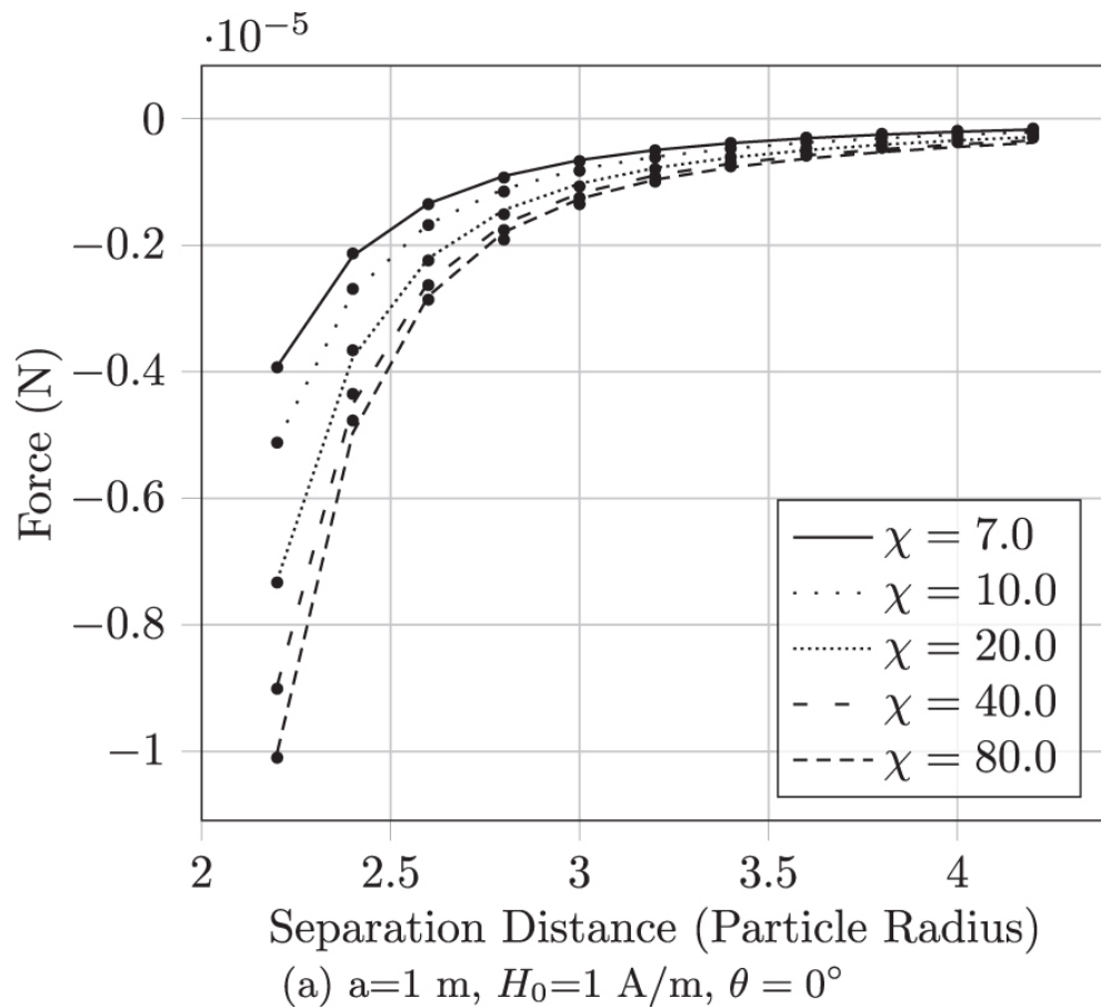
Figure 6. from Anmol Sikka et al 2023 Planet. Sci. J. 4 doi:10.3847/PSJ/ace323 https://dx.doi.org/10.3847/PSJ/ace323 © 2023. The Author(s). Published by the American Astronomical Society.
