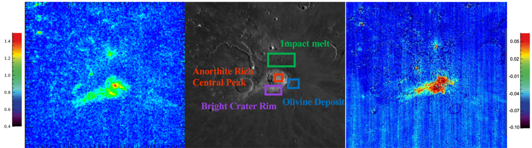
Figure 2. from Elizabeth Czajka et al 2023 Planet. Sci. J. 4 doi:10.3847/PSJ/acdee9 https://dx.doi.org/10.3847/PSJ/acdee9 © 2023. The Author(s). Published by the American Astronomical Society.
