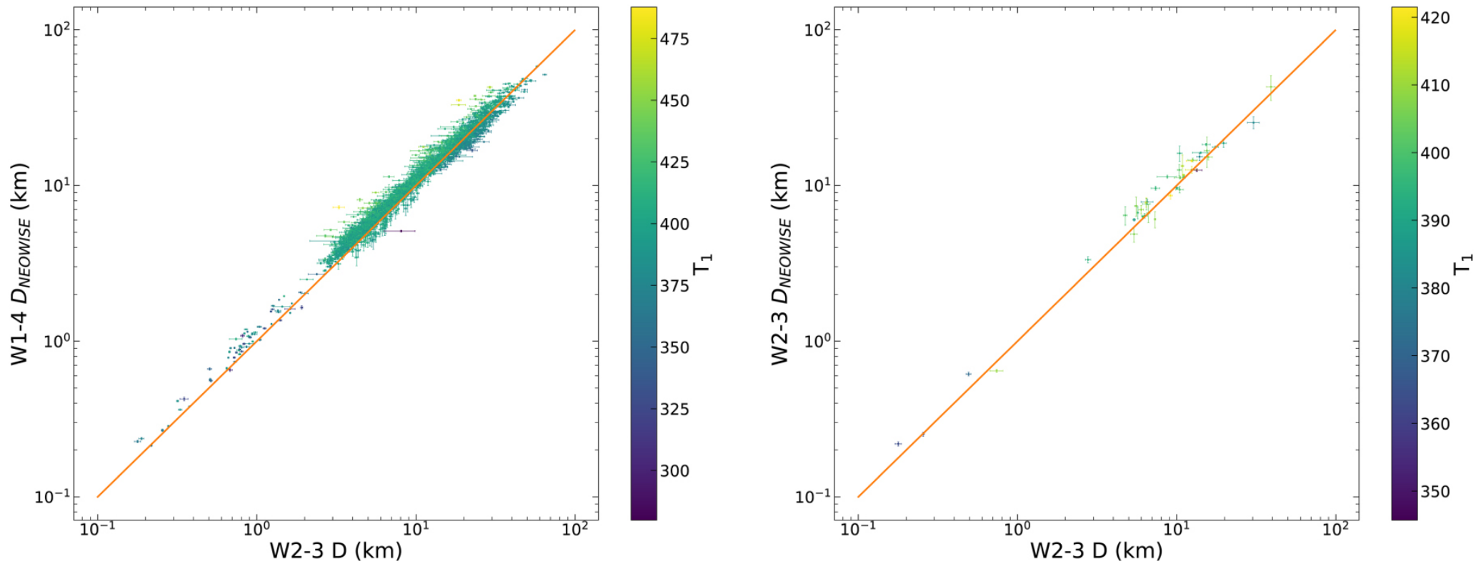
Figure 8. from Emily A. Whittaker et al 2023 Planet. Sci. J. 4 doi:10.3847/PSJ/acc6d2 https://dx.doi.org/10.3847/PSJ/acc6d2 © 2023. The Author(s). Published by the American Astronomical Society.
