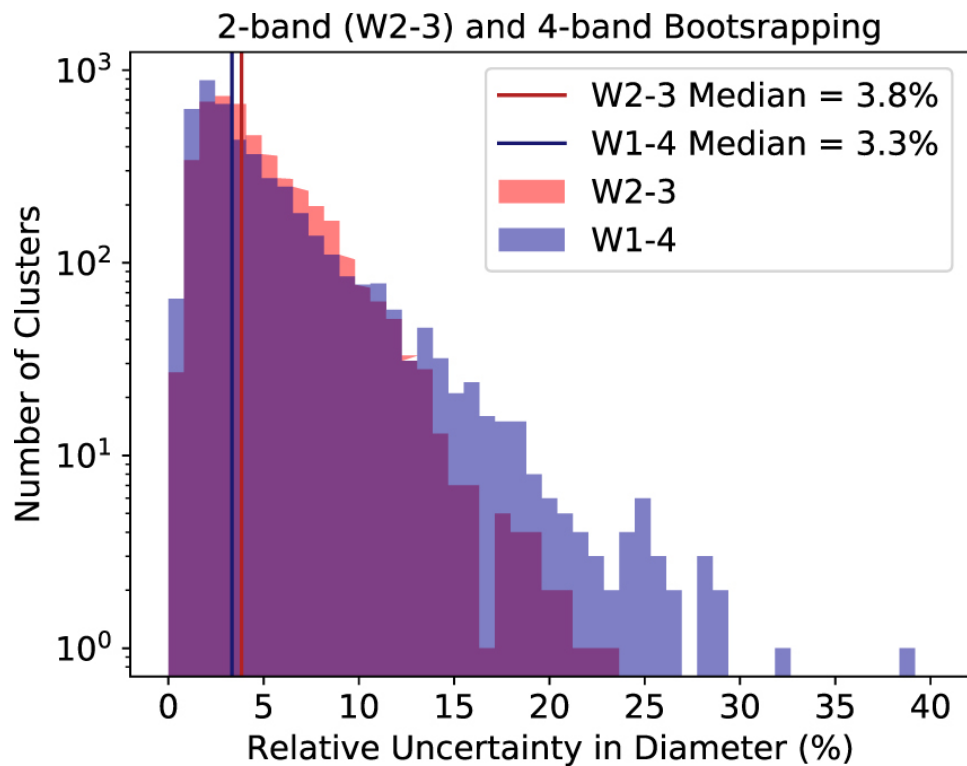
Figure 5. from Emily A. Whittaker et al 2023 Planet. Sci. J. 4 doi:10.3847/PSJ/acc6d2 https://dx.doi.org/10.3847/PSJ/acc6d2 © 2023. The Author(s). Published by the American Astronomical Society.
