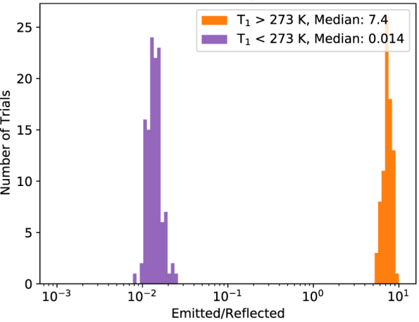
Ratio of Emitted/Reflected Light for Asteroid 10125
