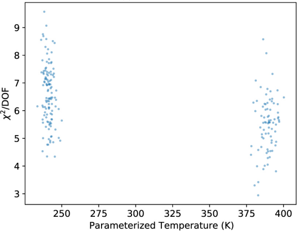
2-band Bootstrapped solution for Asteroid 10125
