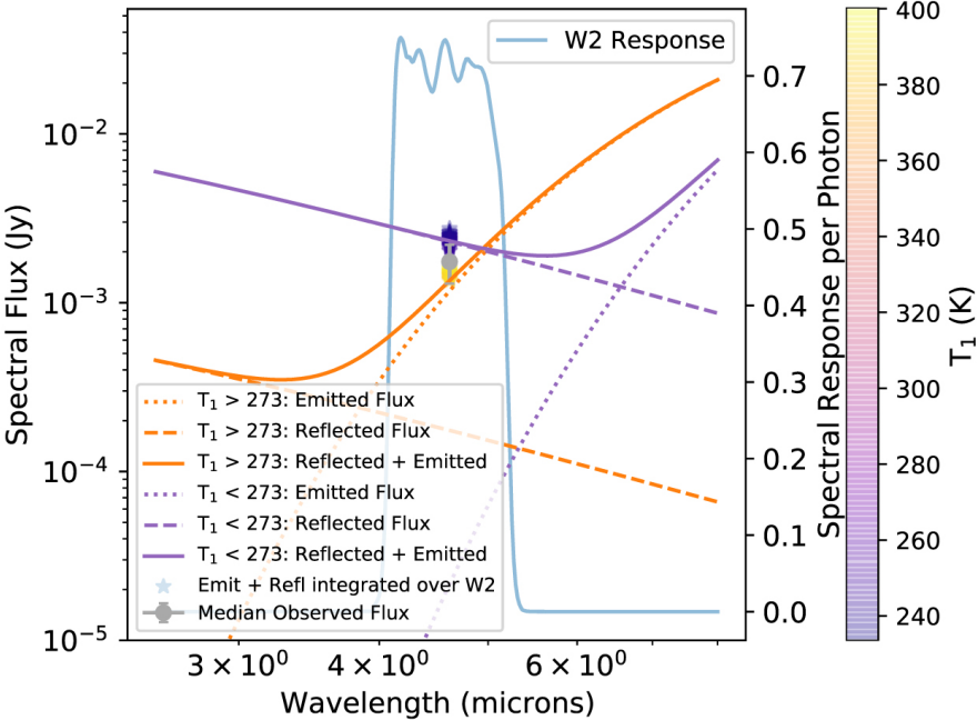
Planck Functions from a 2-band Bootstrapped Solution for W2 for Asteroid 10125
