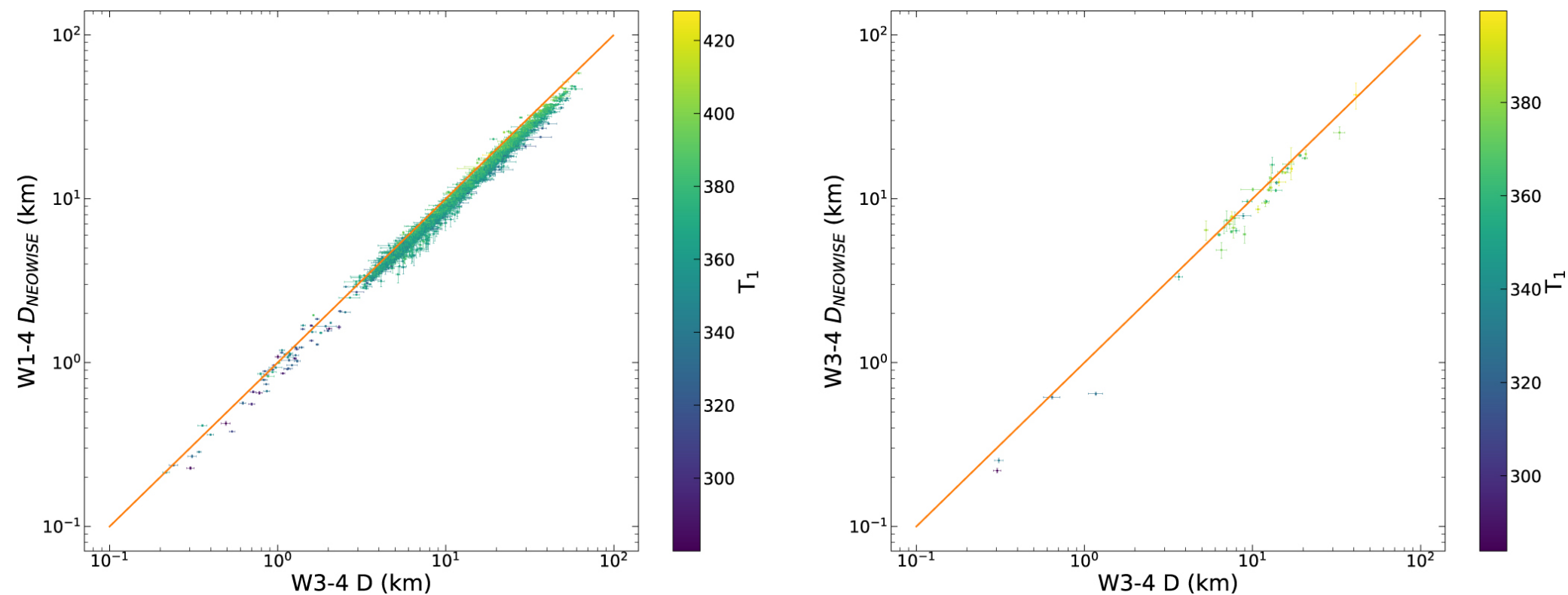
Figure 14. from Emily A. Whittaker et al 2023 Planet. Sci. J. 4 doi:10.3847/PSJ/acc6d2 https://dx.doi.org/10.3847/PSJ/acc6d2 © 2023. The Author(s). Published by the American Astronomical Society.
