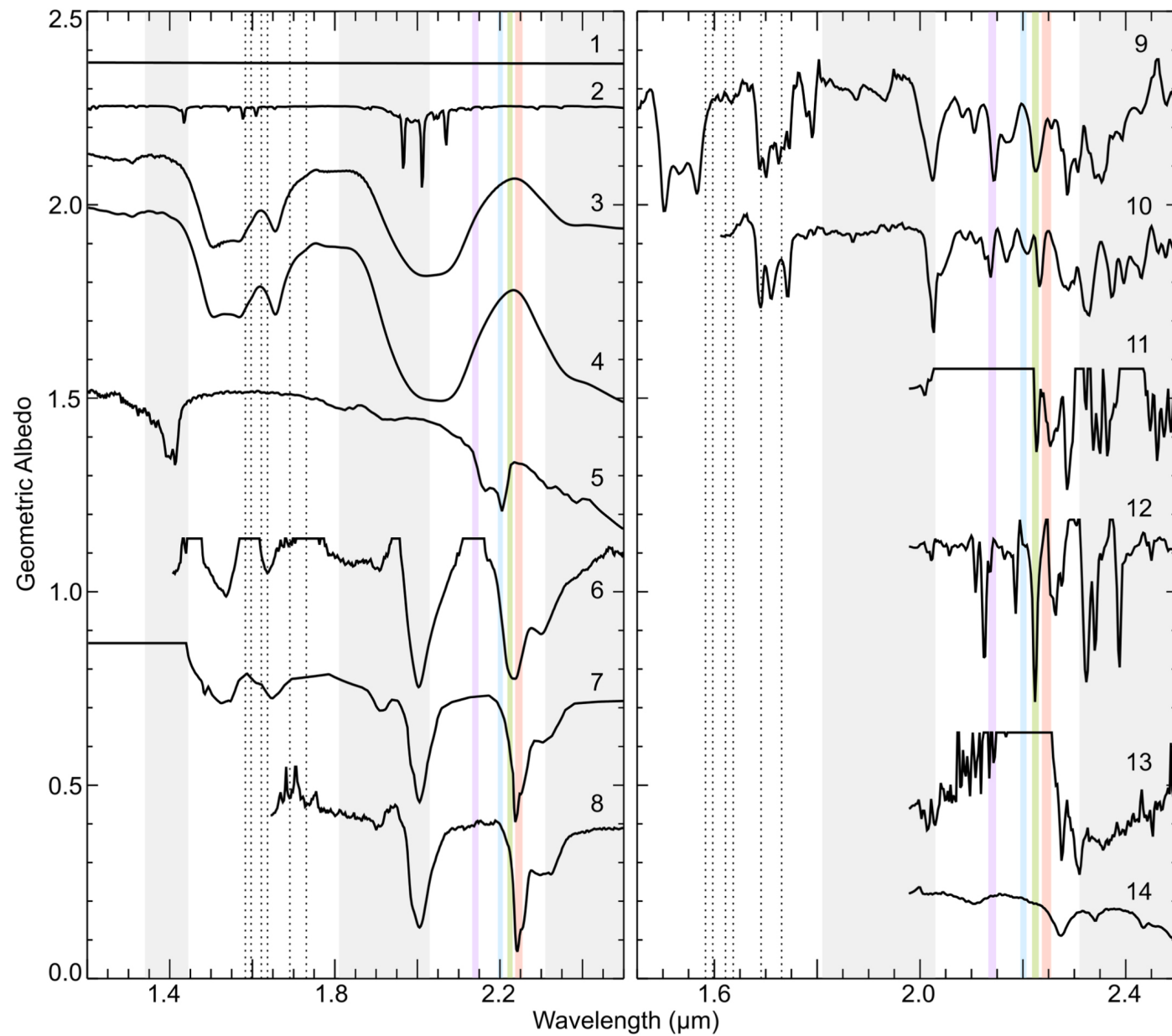
Figure A1. from Richard J. Cartwright et al 2023 Planet. Sci. J. 4 doi:10.3847/PSJ/acbc1f https://dx.doi.org/10.3847/PSJ/acbc1f © 2023. The Author(s). Published by the American Astronomical Society.
