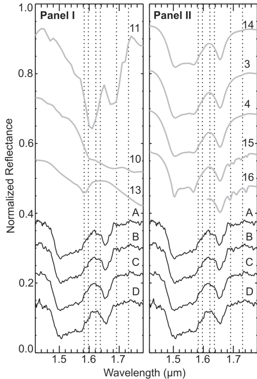
Figure 6. from Richard J. Cartwright et al 2023 Planet. Sci. J. 4 doi:10.3847/PSJ/acbc1f https://dx.doi.org/10.3847/PSJ/acbc1f © 2023. The Author(s). Published by the American Astronomical Society.
