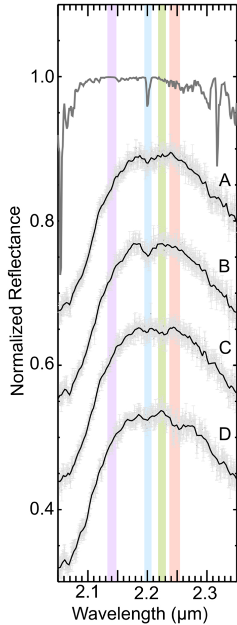
Figure 3. from Richard J. Cartwright et al 2023 Planet. Sci. J. 4 doi:10.3847/PSJ/acbc1f https://dx.doi.org/10.3847/PSJ/acbc1f © 2023. The Author(s). Published by the American Astronomical Society.
