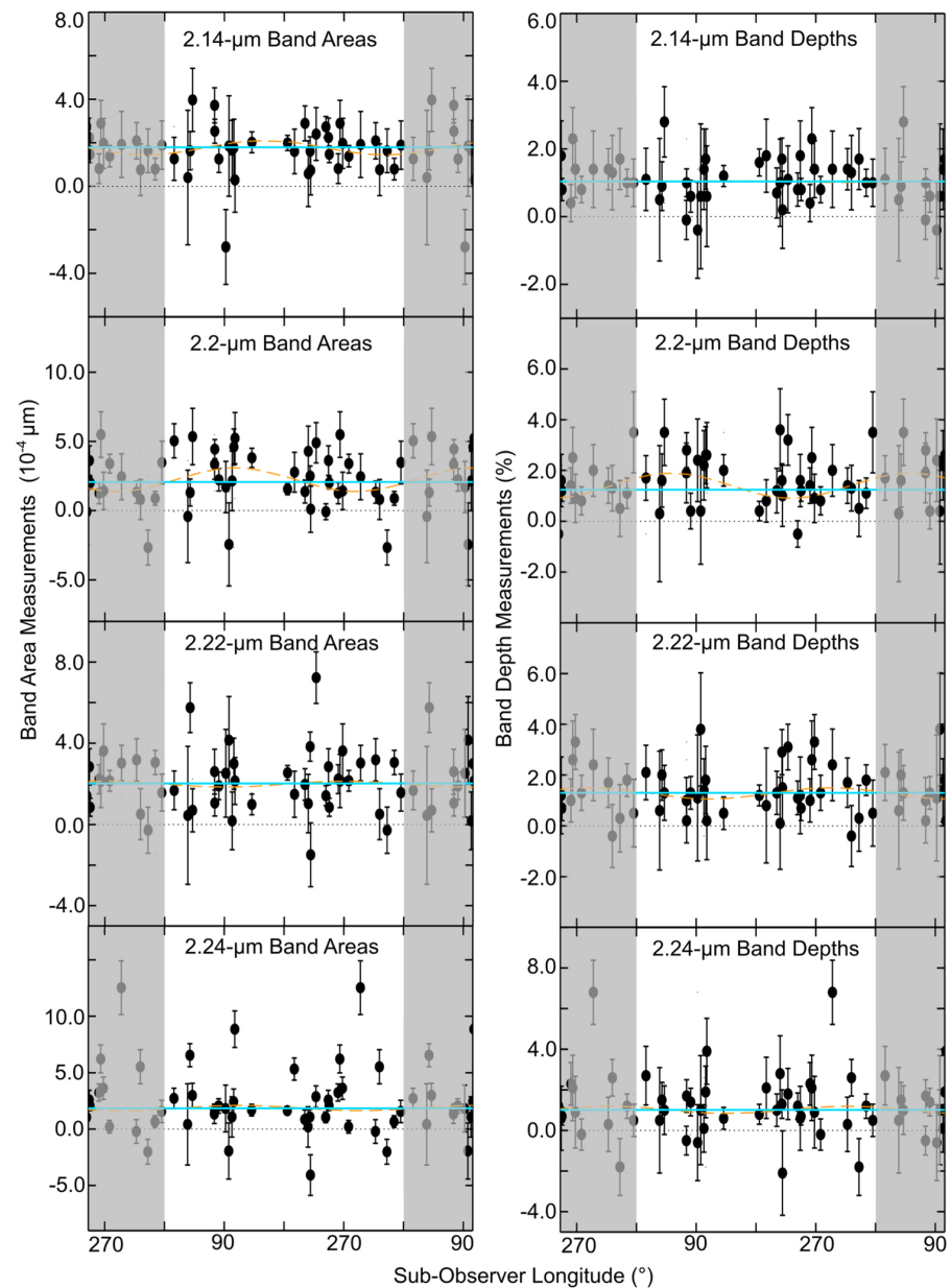
Figure 2. from Richard J. Cartwright et al 2023 Planet. Sci. J. 4 doi:10.3847/PSJ/acbc1f https://dx.doi.org/10.3847/PSJ/acbc1f © 2023. The Author(s). Published by the American Astronomical Society.
