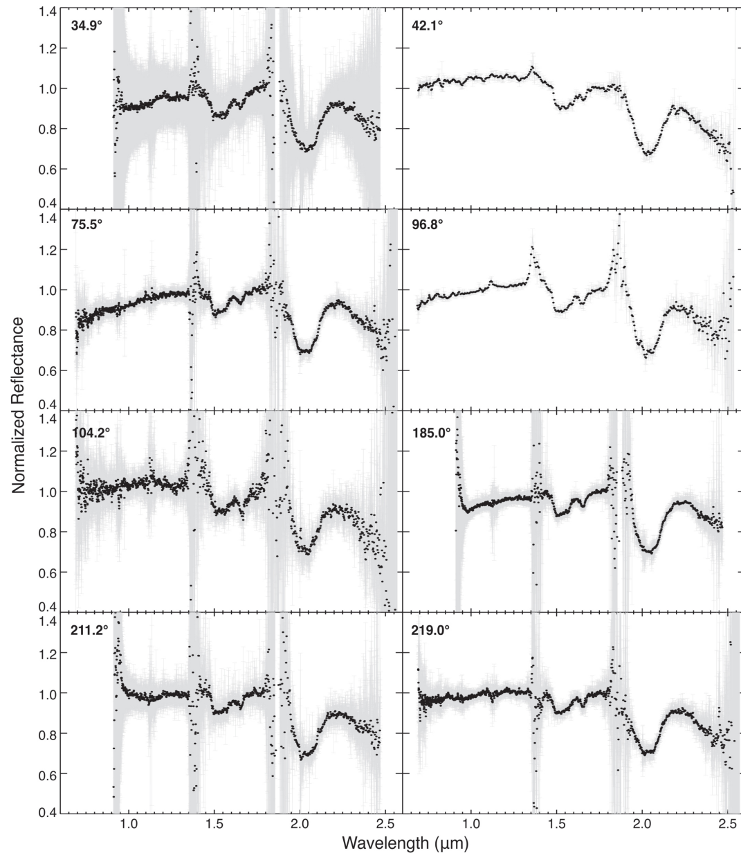
Figure A2. from Richard J. Cartwright et al 2023 Planet. Sci. J. 4 doi:10.3847/PSJ/acbc1f https://dx.doi.org/10.3847/PSJ/acbc1f © 2023. The Author(s). Published by the American Astronomical Society.
