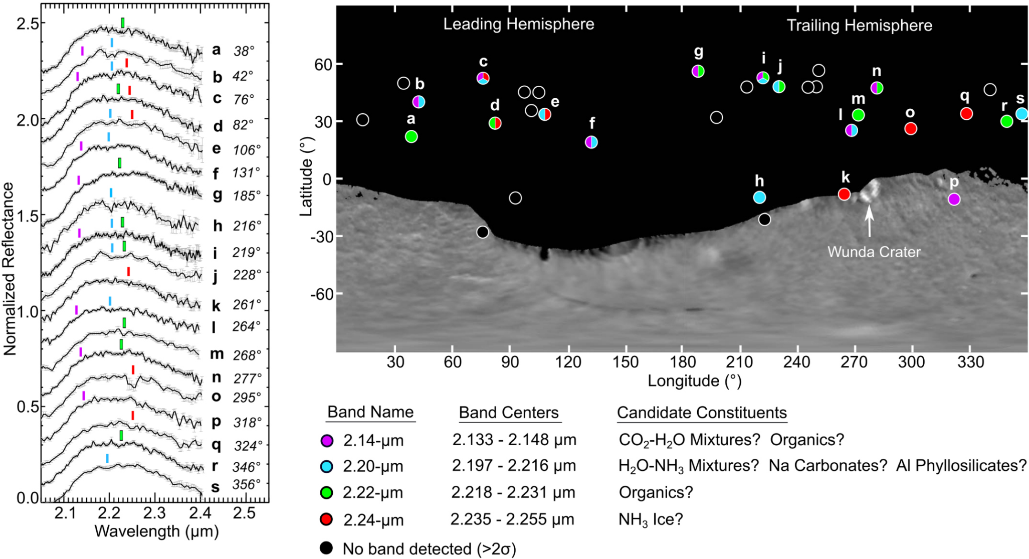
Figure 1. from Richard J. Cartwright et al 2023 Planet. Sci. J. 4 doi:10.3847/PSJ/acbc1f https://dx.doi.org/10.3847/PSJ/acbc1f © 2023. The Author(s). Published by the American Astronomical Society.
