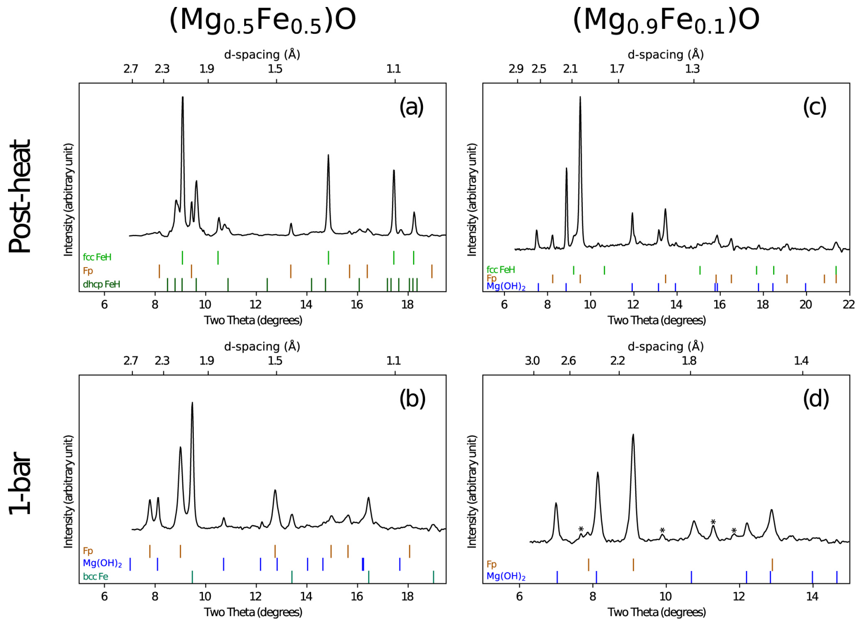
Figure 3. from H. W. Horn et al 2023 Planet. Sci. J. 4 doi:10.3847/PSJ/acab03 https://dx.doi.org/10.3847/PSJ/acab03 © 2023. The Author(s). Published by the American Astronomical Society.
