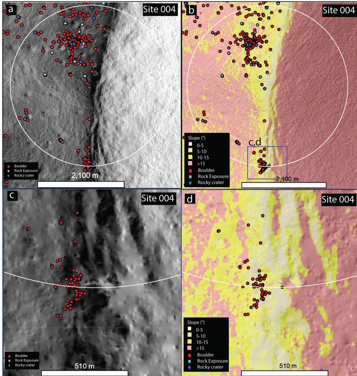
Figure 9. from Sarah. J. Boazman et al 2022 Planet. Sci. J. 3 doi:10.3847/PSJ/aca590 https://dx.doi.org/10.3847/PSJ/aca590 © 2022. The Author(s). Published by the American Astronomical Society.
