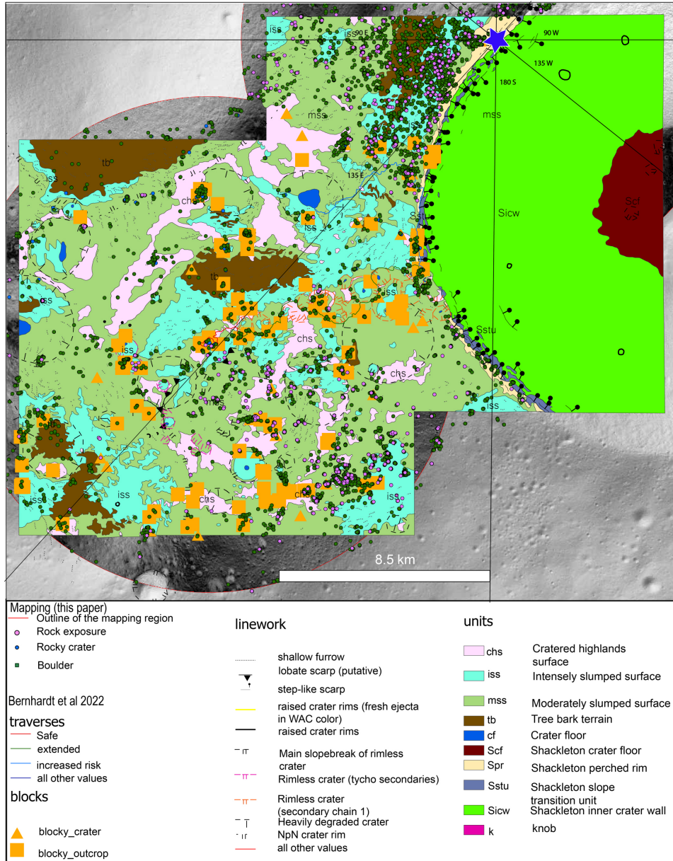
Figure 6. from Sarah. J. Boazman et al 2022 Planet. Sci. J. 3 doi:10.3847/PSJ/aca590 https://dx.doi.org/10.3847/PSJ/aca590 © 2022. The Author(s). Published by the American Astronomical Society.
