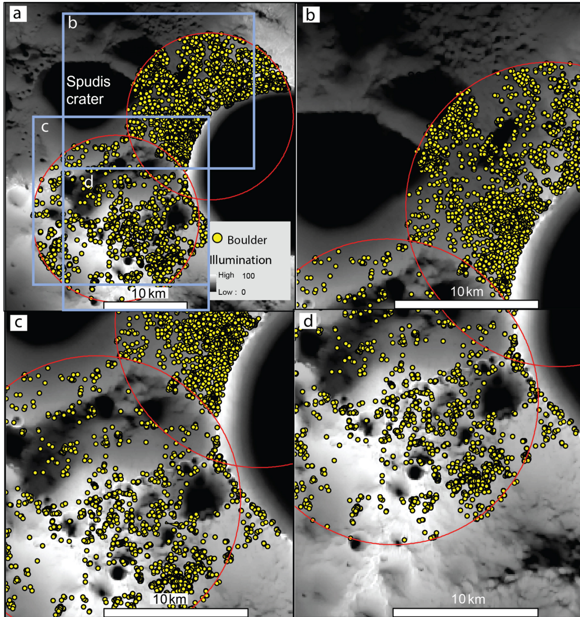
Figure 5. from Sarah. J. Boazman et al 2022 Planet. Sci. J. 3 doi:10.3847/PSJ/aca590 https://dx.doi.org/10.3847/PSJ/aca590 © 2022. The Author(s). Published by the American Astronomical Society.
