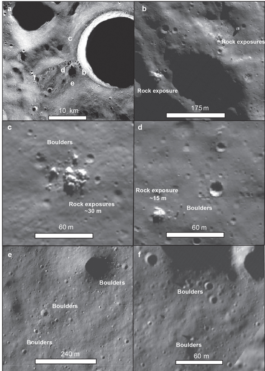
Figure 10. from Sarah. J. Boazman et al 2022 Planet. Sci. J. 3 doi:10.3847/PSJ/aca590 https://dx.doi.org/10.3847/PSJ/aca590 © 2022. The Author(s). Published by the American Astronomical Society.
