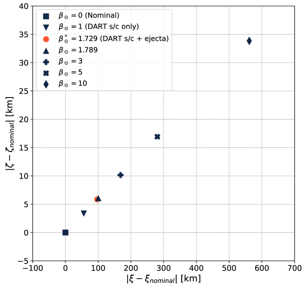
Figure 7. from Rahil Makadia et al 2022 Planet. Sci. J. 3 doi:10.3847/PSJ/ac7de7 https://dx.doi.org/10.3847/PSJ/ac7de7 © 2022. The Author(s). Published by the American Astronomical Society.
