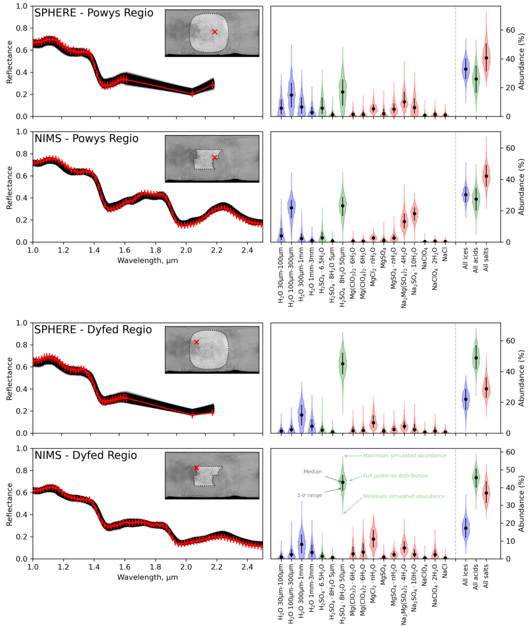
Figure 9. from Oliver King et al 2022 Planet. Sci. J. 3 doi:10.3847/PSJ/ac596d https://dx.doi.org/10.3847/PSJ/ac596d © 2022. The Author(s). Published by the American Astronomical Society.
