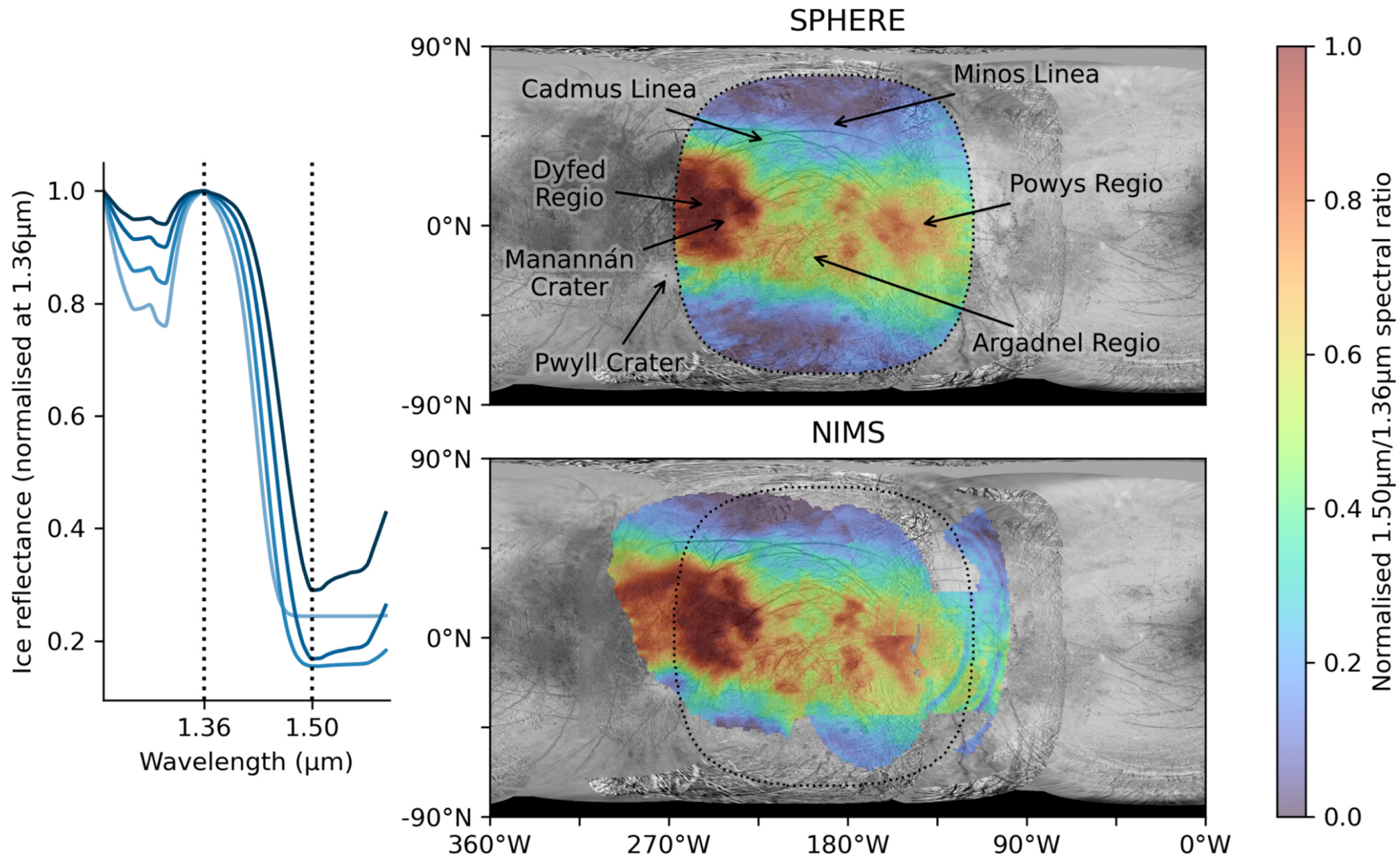
Figure 6. from Oliver King et al 2022 Planet. Sci. J. 3 doi:10.3847/PSJ/ac596d https://dx.doi.org/10.3847/PSJ/ac596d © 2022. The Author(s). Published by the American Astronomical Society.
