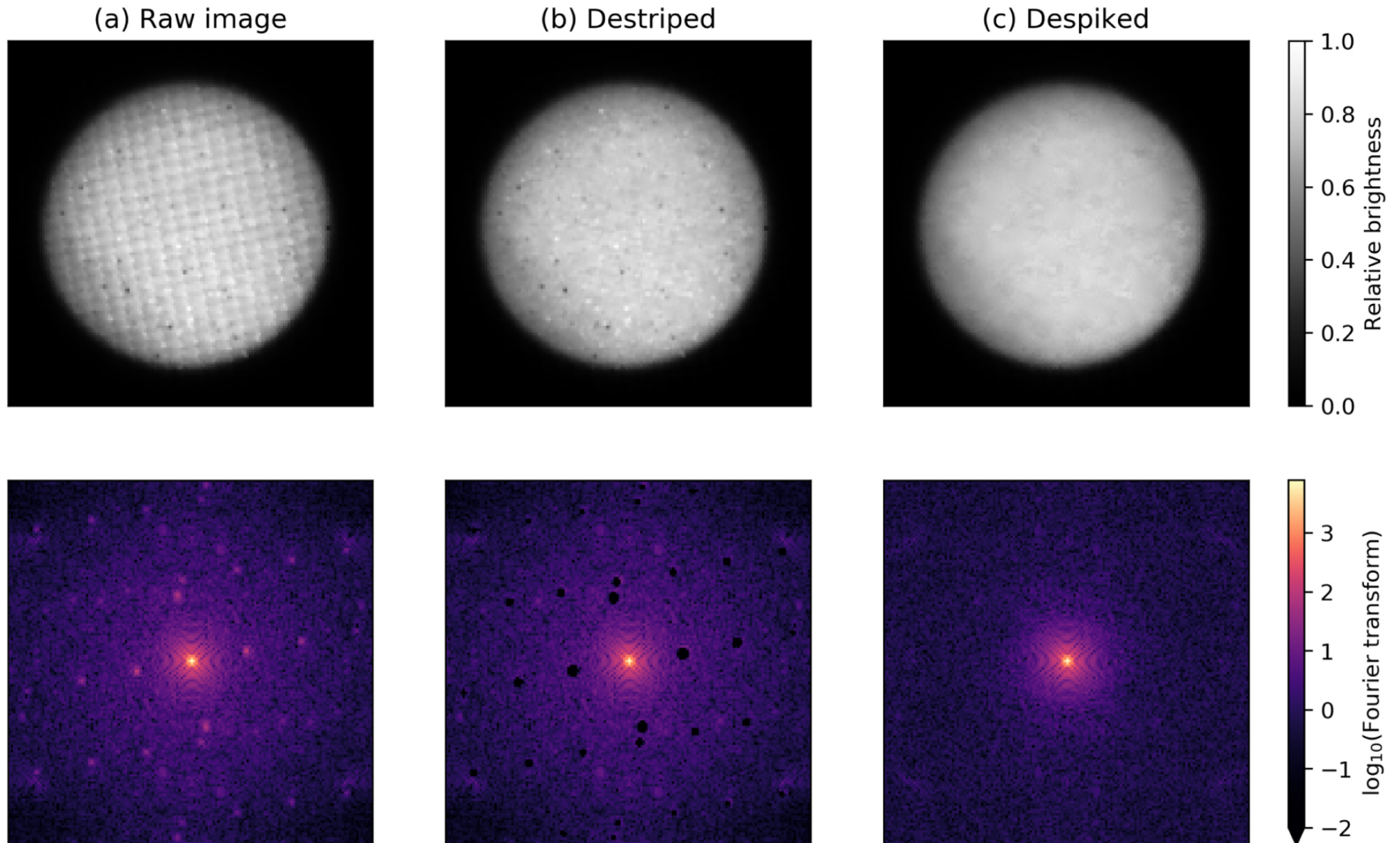
Figure 2. from Oliver King et al 2022 Planet. Sci. J. 3 doi:10.3847/PSJ/ac596d https://dx.doi.org/10.3847/PSJ/ac596d © 2022. The Author(s). Published by the American Astronomical Society.
