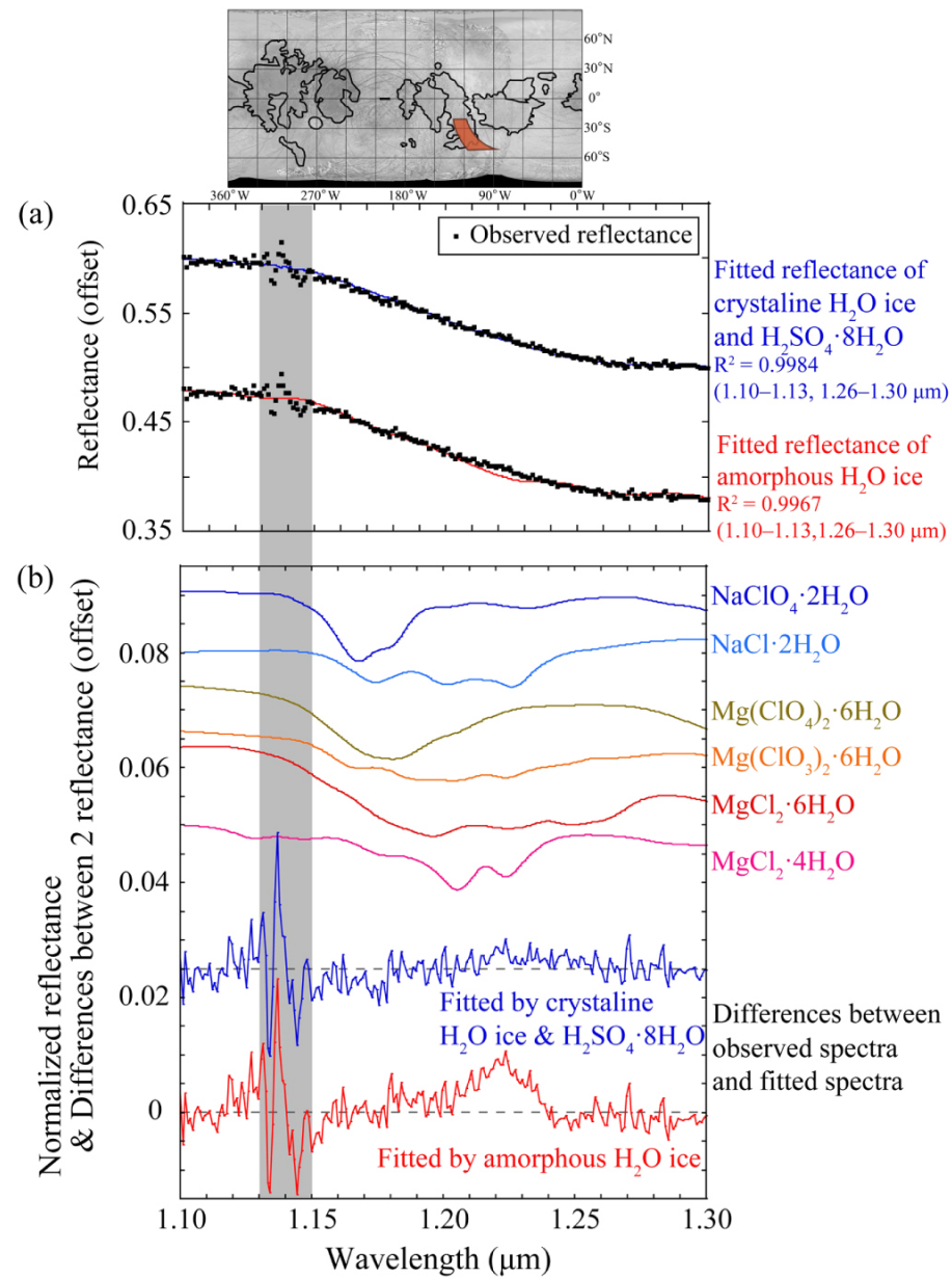
Figure 8. from Shuya Tan et al 2022 Planet. Sci. J. 3 doi:10.3847/PSJ/ac596c https://dx.doi.org/10.3847/PSJ/ac596c © 2022. The Author(s). Published by the American Astronomical Society.
