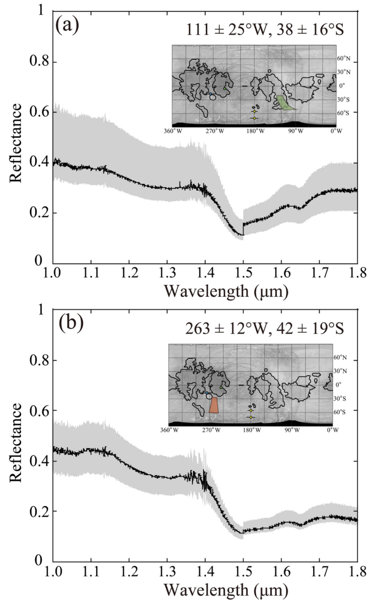
Figure 6. from Shuya Tan et al 2022 Planet. Sci. J. 3 doi:10.3847/PSJ/ac596c https://dx.doi.org/10.3847/PSJ/ac596c © 2022. The Author(s). Published by the American Astronomical Society.
