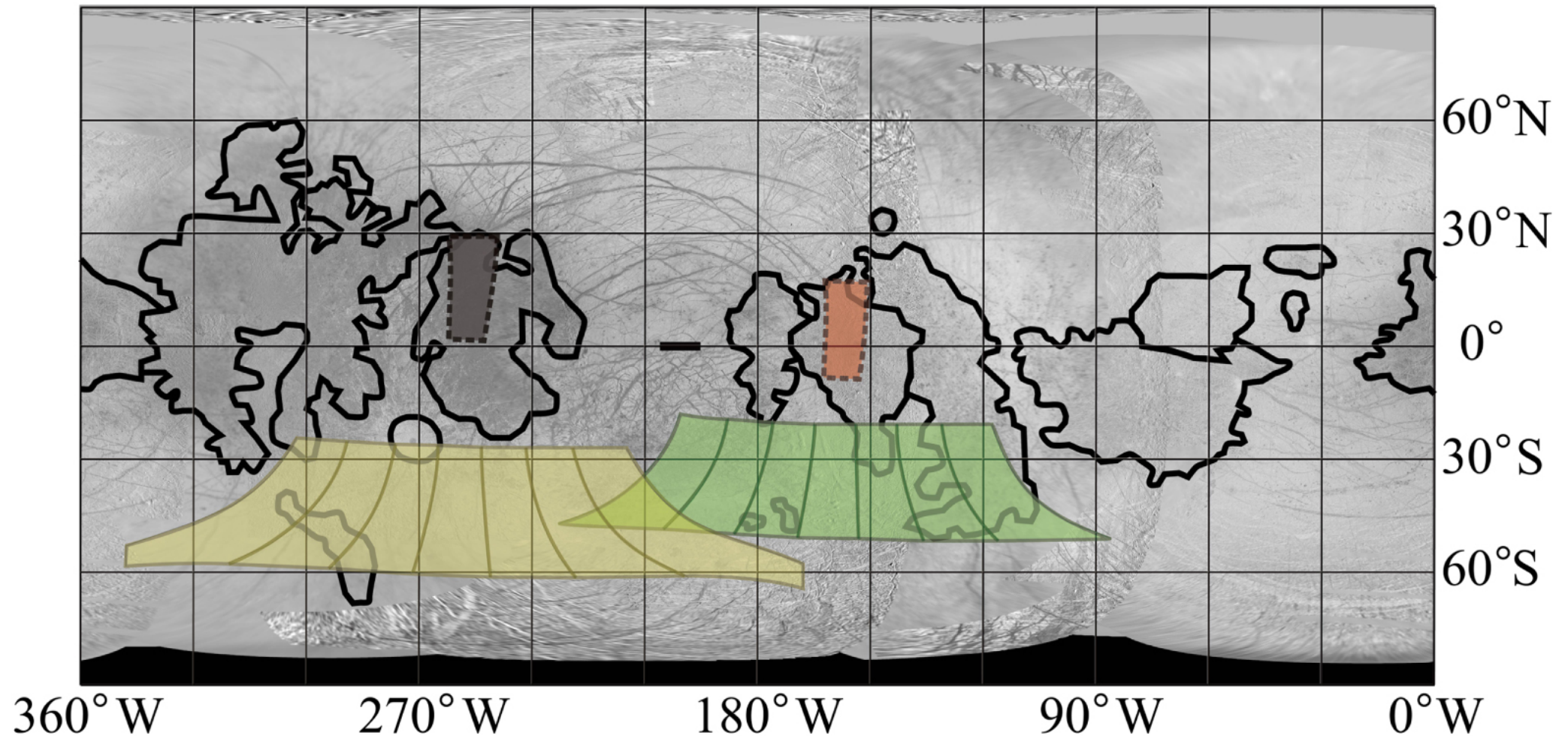
Figure 5. from Shuya Tan et al 2022 Planet. Sci. J. 3 doi:10.3847/PSJ/ac596c https://dx.doi.org/10.3847/PSJ/ac596c © 2022. The Author(s). Published by the American Astronomical Society.
