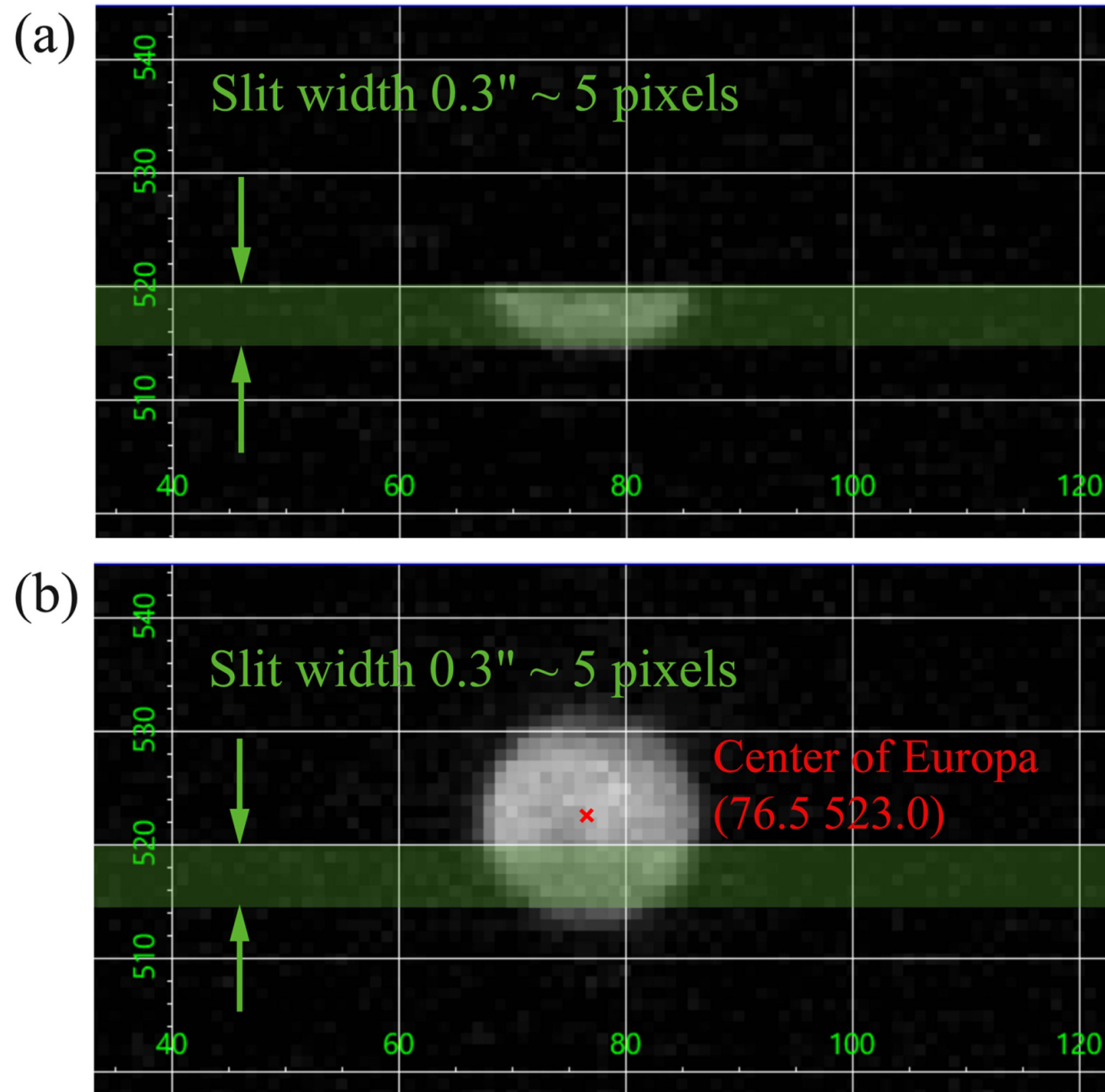
Figure 4. from Shuya Tan et al 2022 Planet. Sci. J. 3 doi:10.3847/PSJ/ac596c https://dx.doi.org/10.3847/PSJ/ac596c © 2022. The Author(s). Published by the American Astronomical Society.
