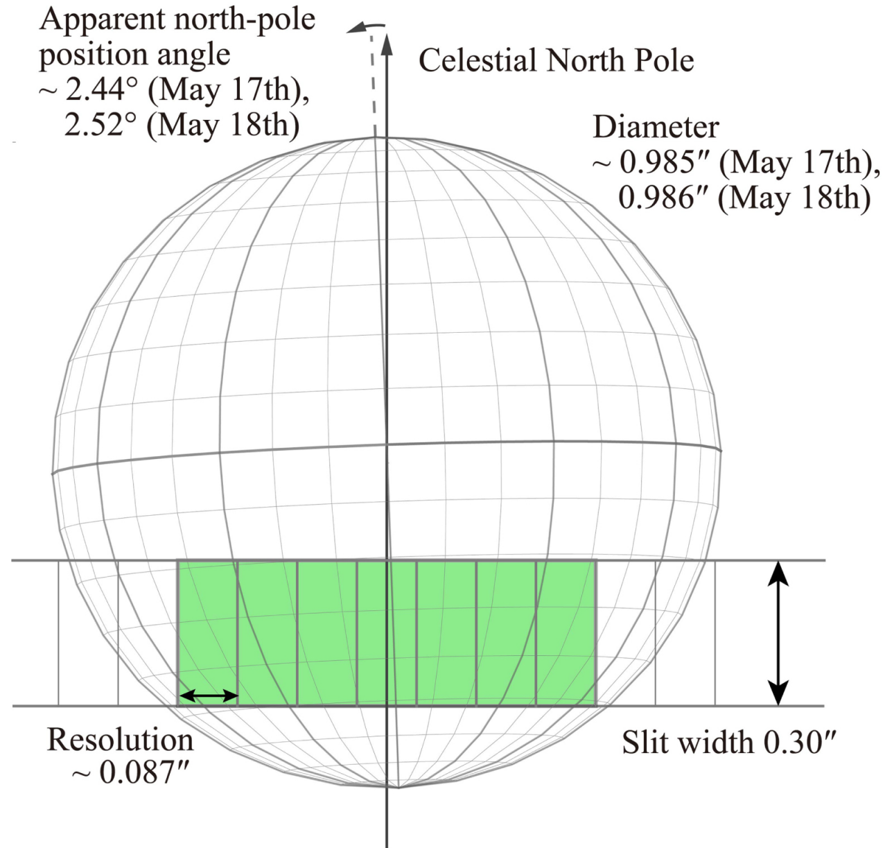
Figure 2. from Shuya Tan et al 2022 Planet. Sci. J. 3 doi:10.3847/PSJ/ac596c https://dx.doi.org/10.3847/PSJ/ac596c © 2022. The Author(s). Published by the American Astronomical Society.
