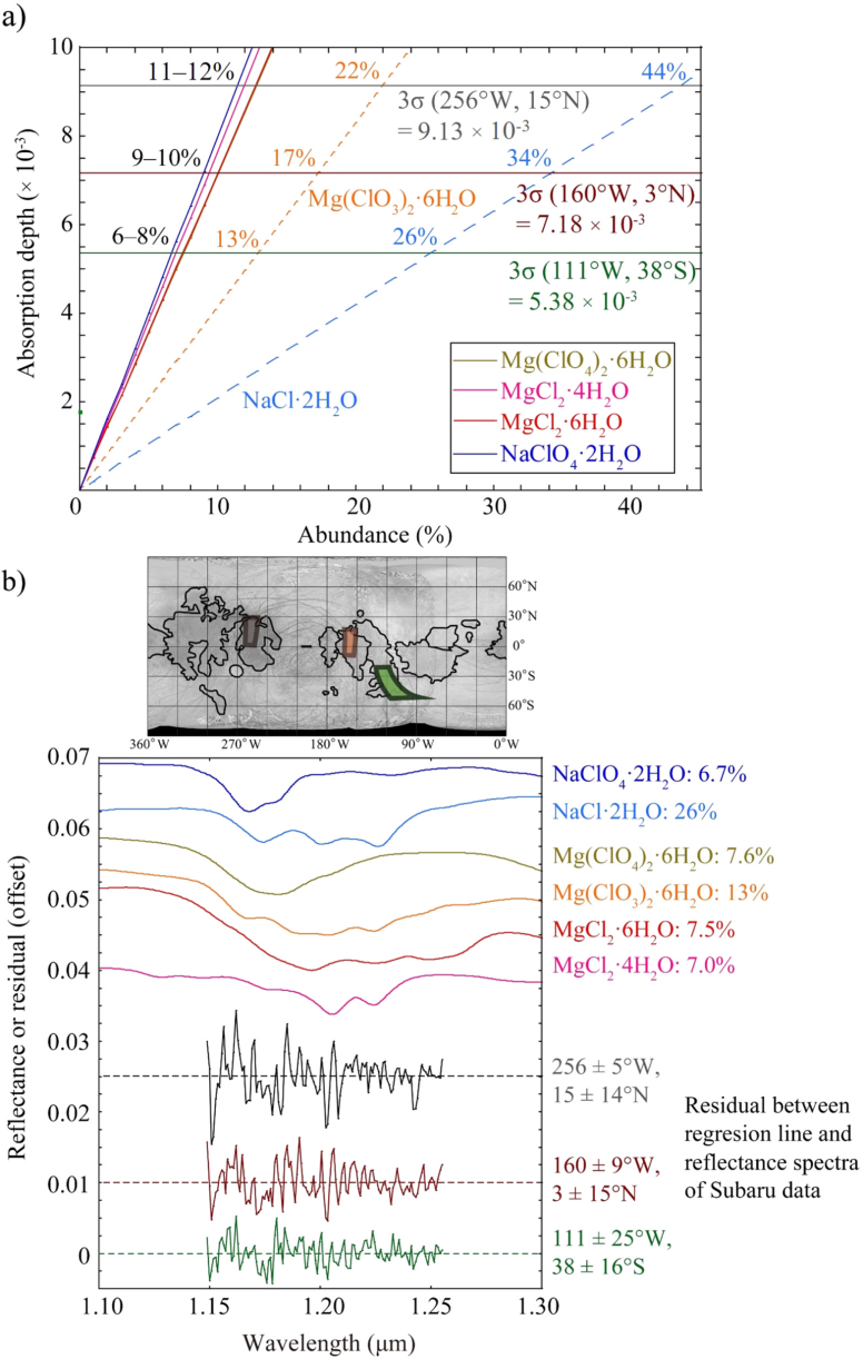
Figure 10. from Shuya Tan et al 2022 Planet. Sci. J. 3 doi:10.3847/PSJ/ac596c https://dx.doi.org/10.3847/PSJ/ac596c © 2022. The Author(s). Published by the American Astronomical Society.
