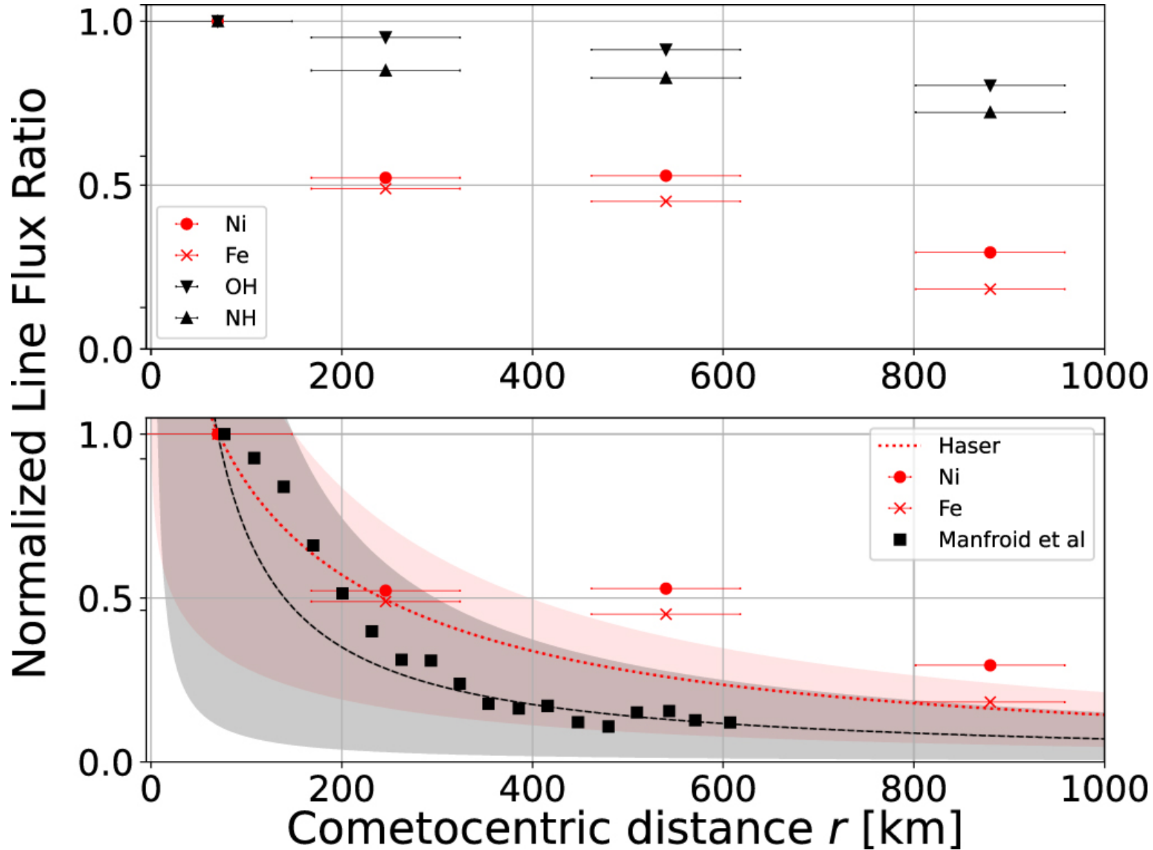
Figure 9. from S. J. Bromley et al 2021 Planet. Sci. J. 2 doi:10.3847/PSJ/ac2dff https://dx.doi.org/10.3847/PSJ/ac2dff © 2021. The Author(s). Published by the American Astronomical Society.
