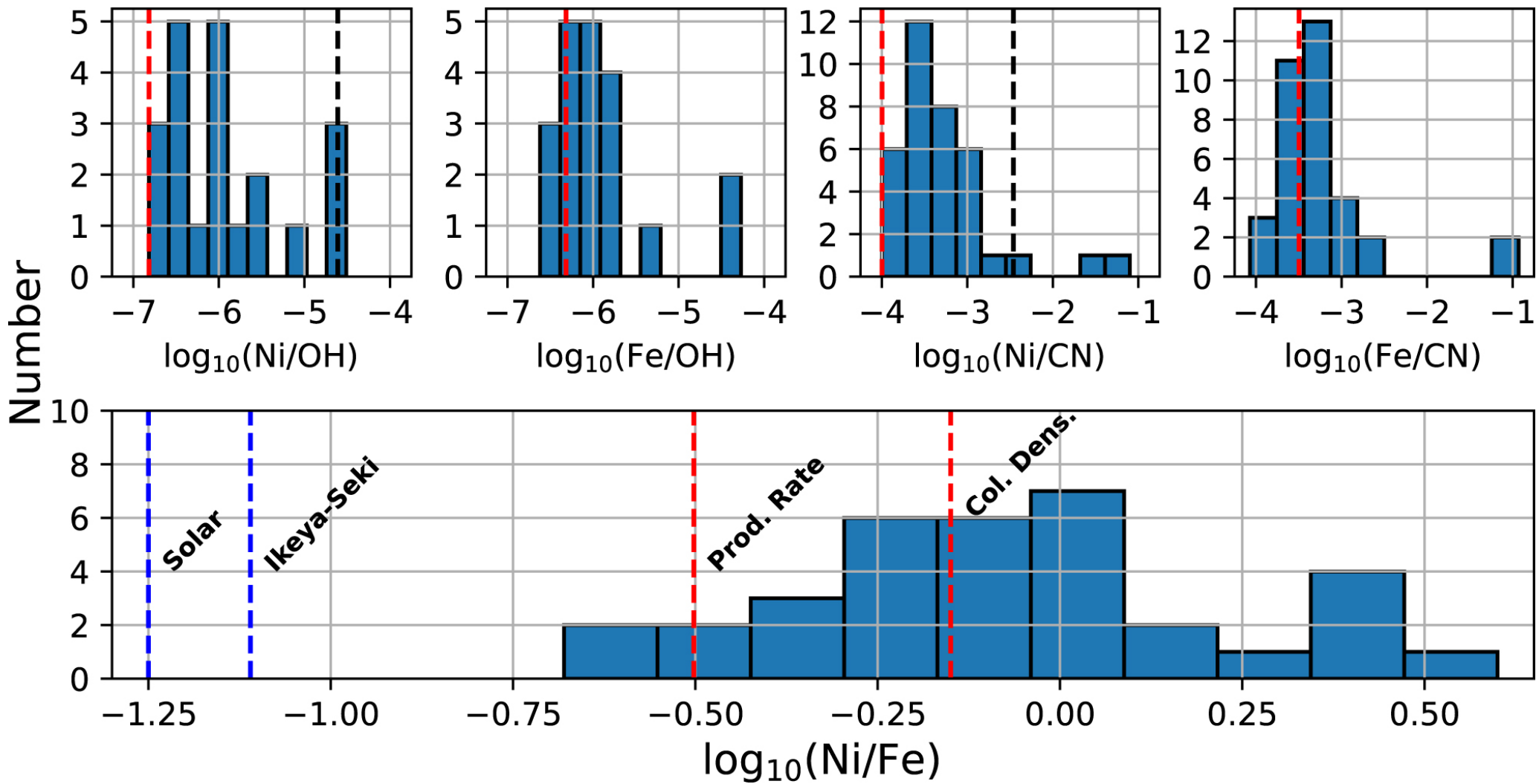
Figure 8. from S. J. Bromley et al 2021 Planet. Sci. J. 2 doi:10.3847/PSJ/ac2dff https://dx.doi.org/10.3847/PSJ/ac2dff © 2021. The Author(s). Published by the American Astronomical Society.
