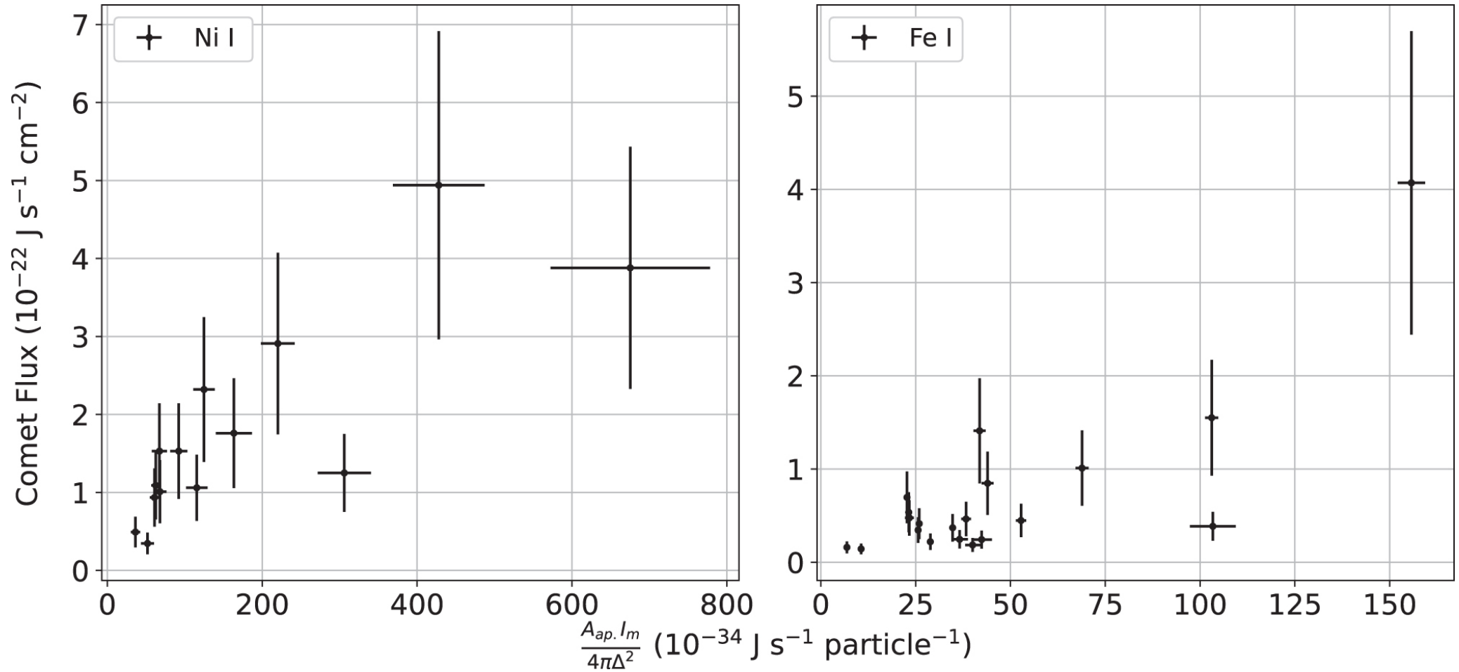
Figure 7. from S. J. Bromley et al 2021 Planet. Sci. J. 2 doi:10.3847/PSJ/ac2dff https://dx.doi.org/10.3847/PSJ/ac2dff © 2021. The Author(s). Published by the American Astronomical Society.
