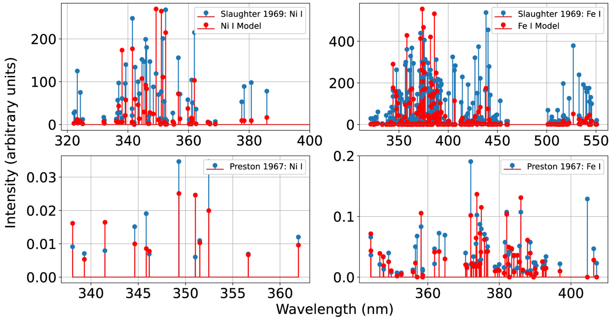
Figure 4. from S. J. Bromley et al 2021 Planet. Sci. J. 2 doi:10.3847/PSJ/ac2dff https://dx.doi.org/10.3847/PSJ/ac2dff © 2021. The Author(s). Published by the American Astronomical Society.
