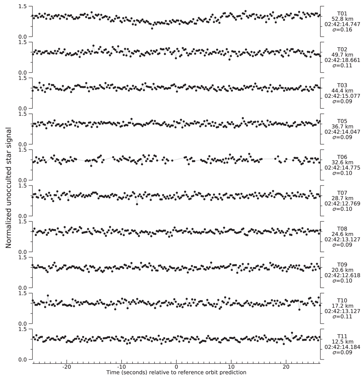
Figure 9. from Size and Shape of (11351) Leucus from Five Occultations null 2021 PSJ 2 202 doi:10.3847/PSJ/ac1f9b https://dx.doi.org/10.3847/PSJ/ac1f9b © 2021. The Author(s). Published by the American Astronomical Society.
