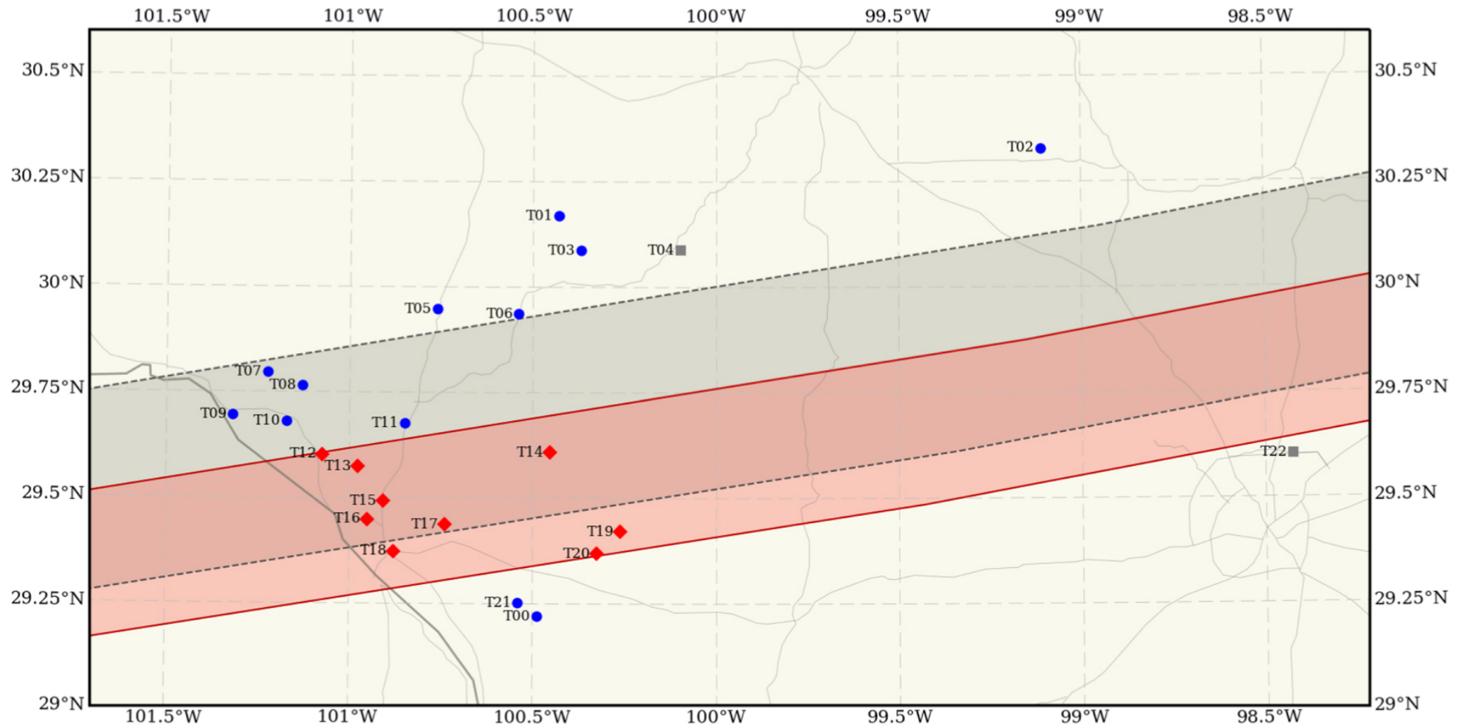
Figure 8. from Size and Shape of (11351) Leucus from Five Occultations null 2021 PSJ 2 202 doi:10.3847/PSJ/ac1f9b https://dx.doi.org/10.3847/PSJ/ac1f9b © 2021. The Author(s). Published by the American Astronomical Society.
