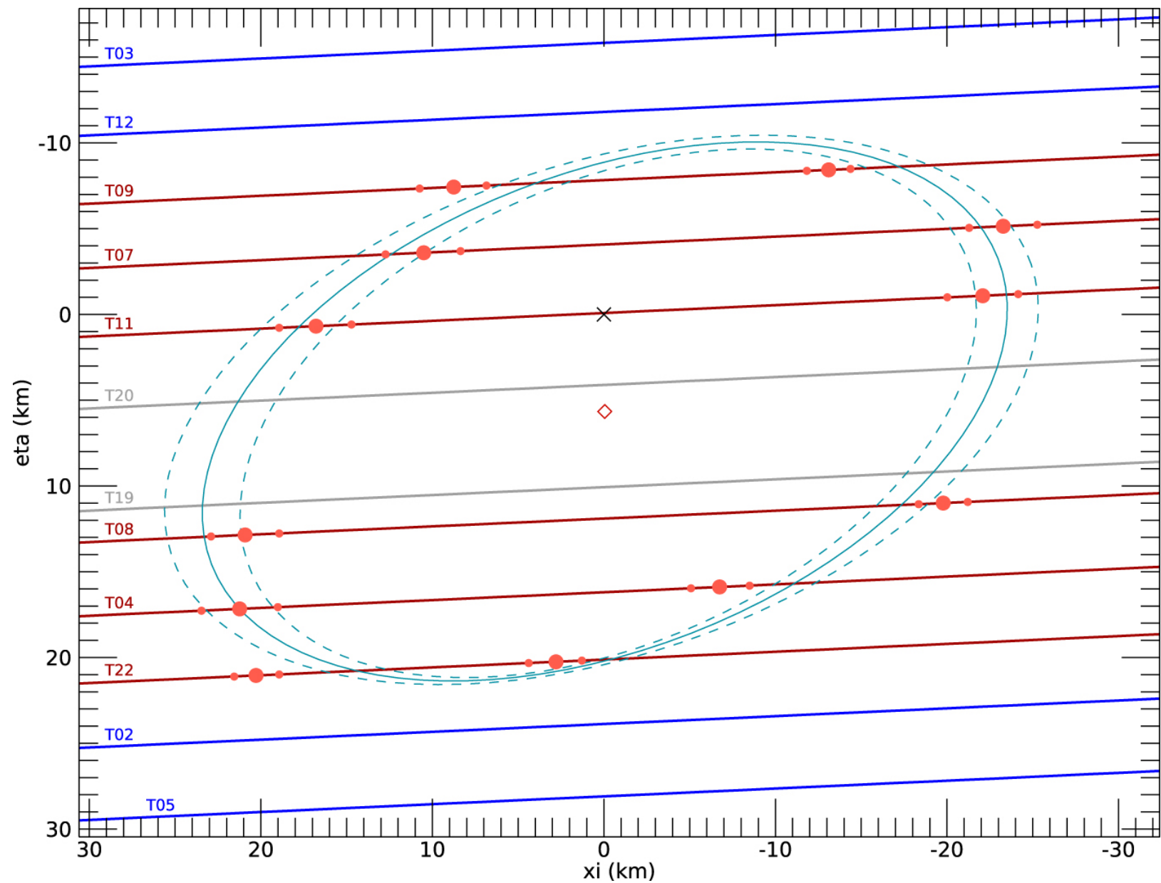
Figure 7. from Size and Shape of (11351) Leucus from Five Occultations null 2021 PSJ 2 202 doi:10.3847/PSJ/ac1f9b https://dx.doi.org/10.3847/PSJ/ac1f9b © 2021. The Author(s). Published by the American Astronomical Society.
