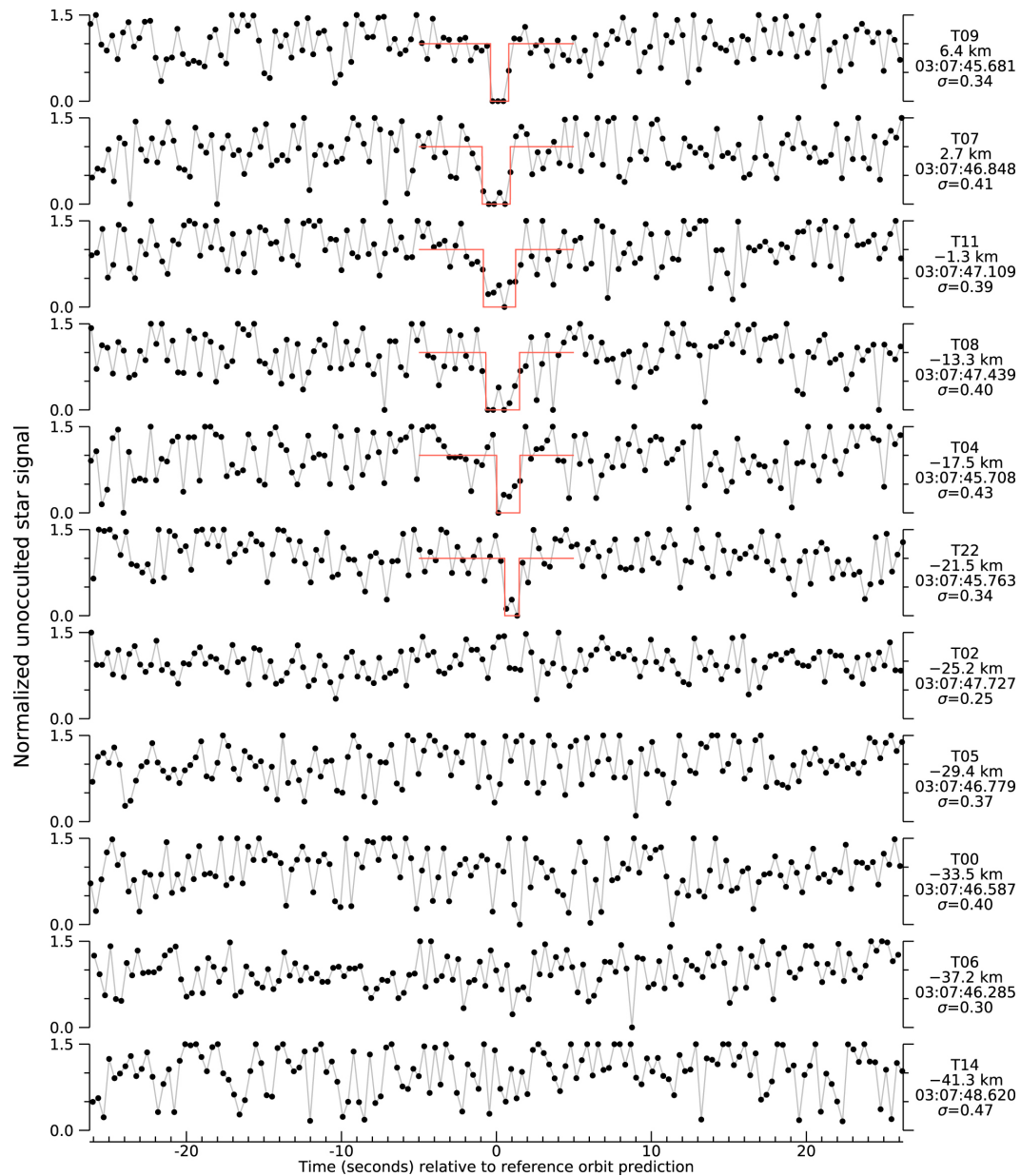
Figure 6. from Size and Shape of (11351) Leucus from Five Occultations null 2021 PSJ 2 202 doi:10.3847/PSJ/ac1f9b https://dx.doi.org/10.3847/PSJ/ac1f9b © 2021. The Author(s). Published by the American Astronomical Society.
