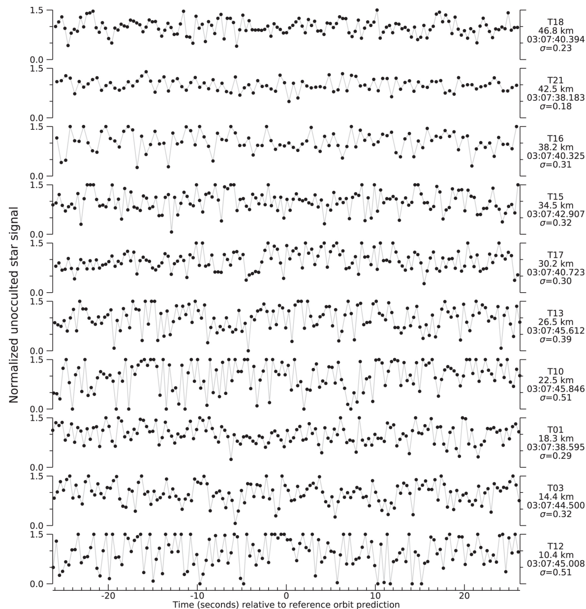
Figure 5. from Size and Shape of (11351) Leucus from Five Occultations null 2021 PSJ 2 202 doi:10.3847/PSJ/ac1f9b https://dx.doi.org/10.3847/PSJ/ac1f9b © 2021. The Author(s). Published by the American Astronomical Society.
