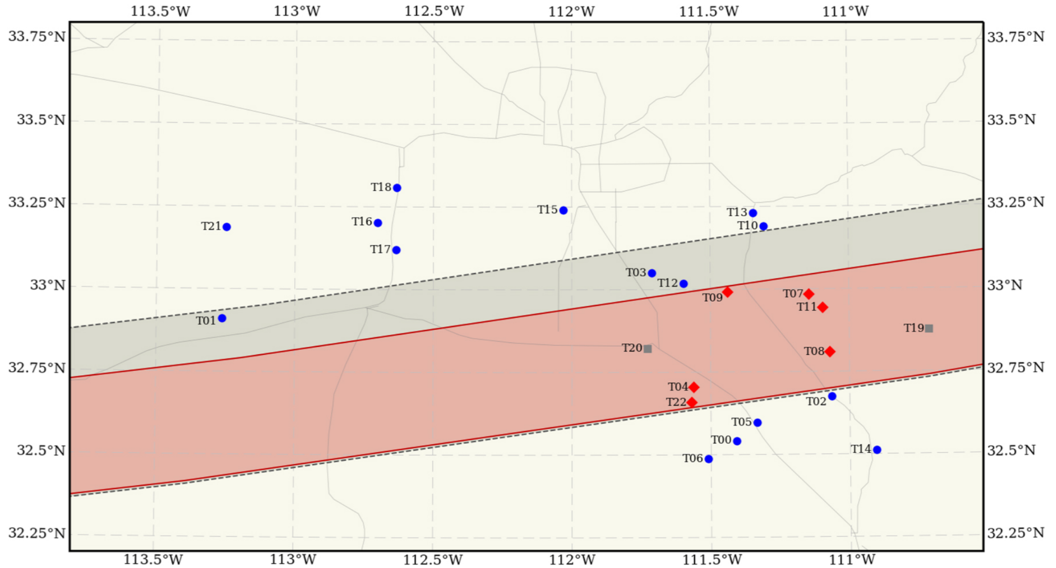
Figure 4. from Size and Shape of (11351) Leucus from Five Occultations null 2021 PSJ 2 202 doi:10.3847/PSJ/ac1f9b https://dx.doi.org/10.3847/PSJ/ac1f9b © 2021. The Author(s). Published by the American Astronomical Society.
