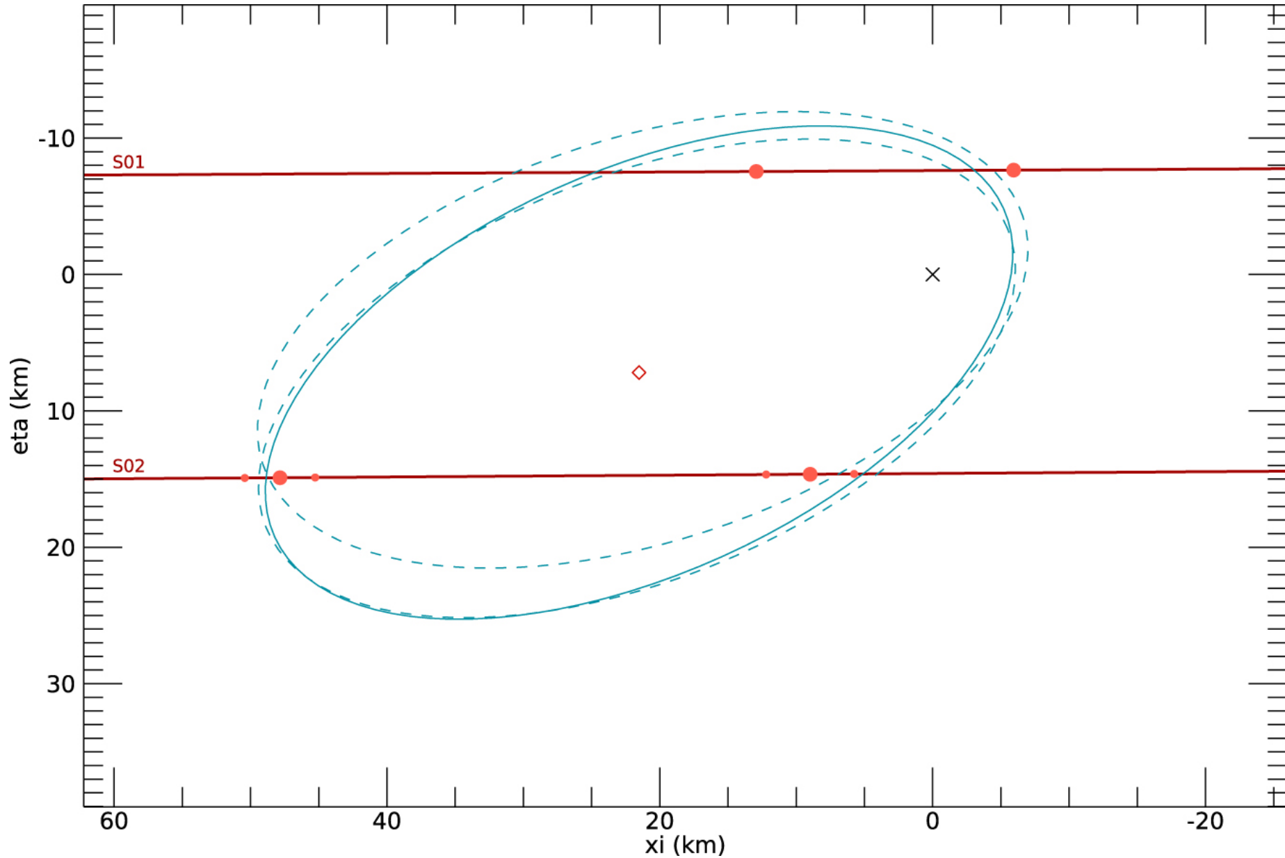
Figure 3. from Size and Shape of (11351) Leucus from Five Occultations null 2021 PSJ 2 202 doi:10.3847/PSJ/ac1f9b https://dx.doi.org/10.3847/PSJ/ac1f9b © 2021. The Author(s). Published by the American Astronomical Society.
