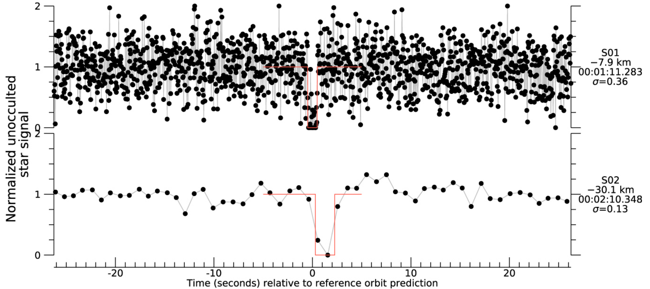
Figure 2. from Size and Shape of (11351) Leucus from Five Occultations null 2021 PSJ 2 202 doi:10.3847/PSJ/ac1f9b https://dx.doi.org/10.3847/PSJ/ac1f9b © 2021. The Author(s). Published by the American Astronomical Society.
