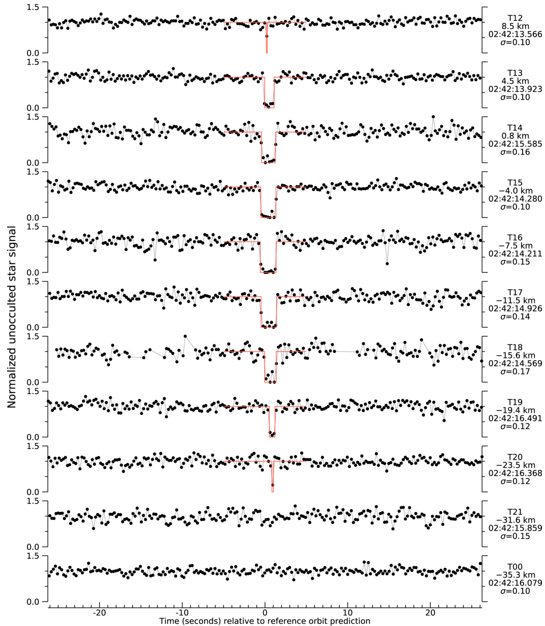
Figure 10. from Size and Shape of (11351) Leucus from Five Occultations null 2021 PSJ 2 202 doi:10.3847/PSJ/ac1f9b https://dx.doi.org/10.3847/PSJ/ac1f9b © 2021. The Author(s). Published by the American Astronomical Society.
